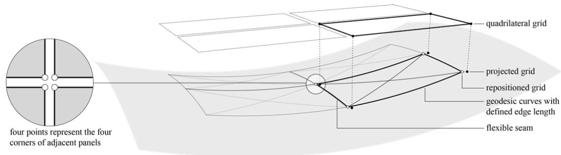
Fig. 9: Modelling process: A quadrilateral point grid is projected onto the target surface. The projected grid is then adjusted to fulfill the expected geodesic-length requirements. Additionally, a seam is simulated by individually modelling each corner of every panel. The resulting four points at each intersection can move independently.
