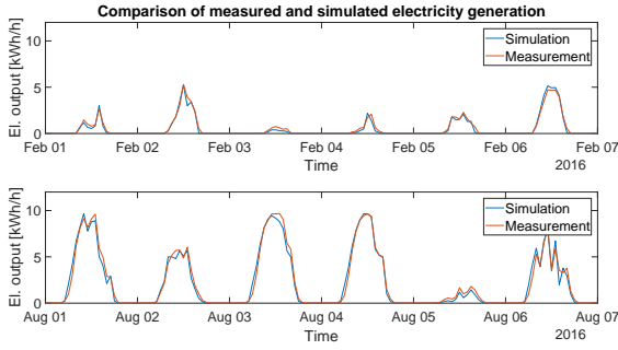
Fig. 2: Measured and simulated generated electricity of the 14\text{ kW}_p PV system located in Munich for two weeks in 2016 using PWX 500 PV module (49 W)
