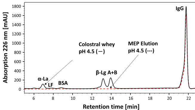
Fig. 11. RP-HPLC chromatograms of the isolation process at highest scale MEP/MMC (8800 mL/300 mL), Colostrum whey sample (solid), MEP primary elution fraction at pH 4.5 (dotted).
