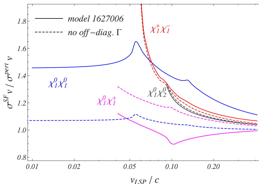
Figure 4. Enhancement factors (\sigma^{\text{SF}}v)/(\sigma^{\text{pert}}v) in the four most relevant two-particle channels \chi_1^0\chi_1^0 , \chi_1^+\chi_1^- , \chi_1^0\chi_2^0 and \chi_1^0\chi_1^+ of Snowmass model 1627006. The enhancement factor for the additionally relevant channel \chi_1^0\chi_1^- agrees with the one for the \chi_1^0\chi_1^+ pair. Solid lines refer to the calculation of the Sommerfeld-enhanced rates with off-diagonal terms in the annihilation matrices properly included. Dashed curves show the enhancement when the off-diagonal annihilation rates are neglected.
