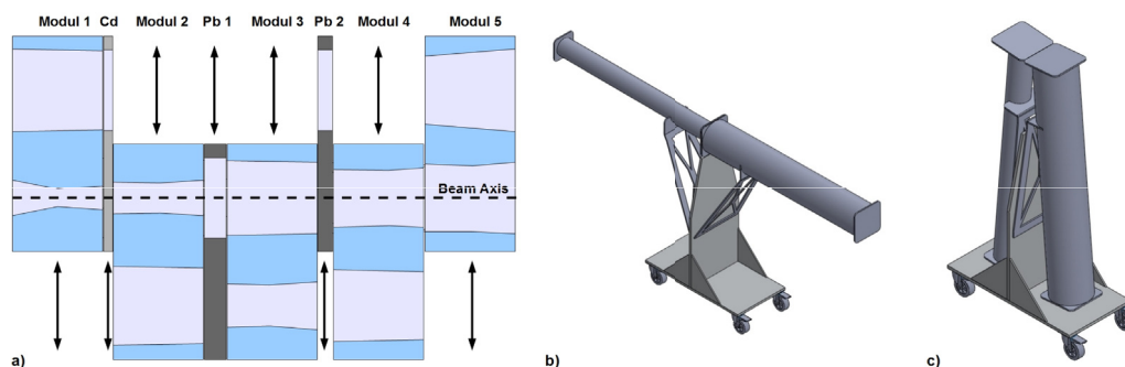
Fig. 2. a) Collimator with movable modules (Modul 1 to Modul 5) enabling for different L/D ratios and additional filters (e.g. Cd, Pb 1, Pb 2) directly included inside the modular collimator; b) proposed layout of a flight tube in operating position, temporarily placed inside the MEDAPP chamber; c) flight tube in storage position.
