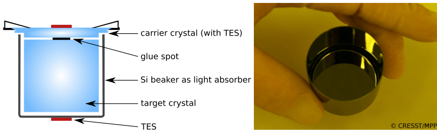
Fig. 5 Beaker light detectors. Left: CRESST beaker-module holding scheme including glued TES-carrier to complete a 4 \pi -veto. Right: polished silicon beaker (height 40 mm, diameter 40 mm, thickness 0.4 mm) milled from single crystal material (Color figure online)
