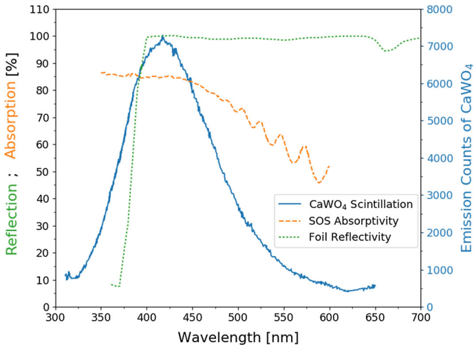
Fig. 2 CaWO 4 scintillation spectrum (solid blue line), wavelength-dependent reflectivity of the scintillating foil (dotted green line), and absorption of SOS wafers (dashed orange line) [5] (Color figure online)
