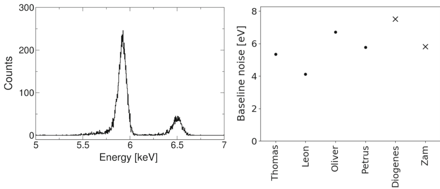
Fig. 4 Left: 55 Mn K α /K β lines observed in CRESST-II light detector Leon . Right: baseline resolutions achieved by the CRESST-II light detectors equipped with 55 Fe sources for direct calibration. Dots: standard light detectors. Crosses: beaker light detectors
