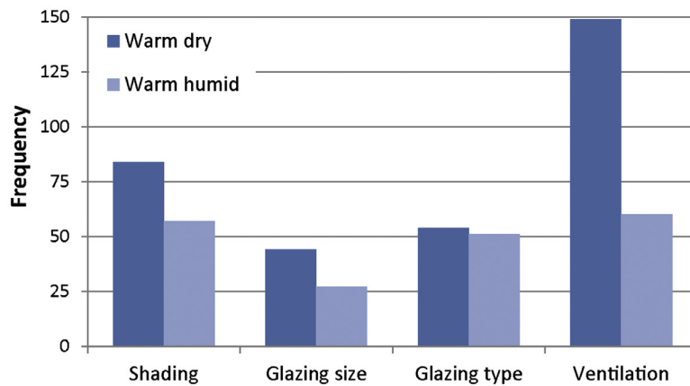
Fig. 3. Number of results per strategy and main climate groups.
