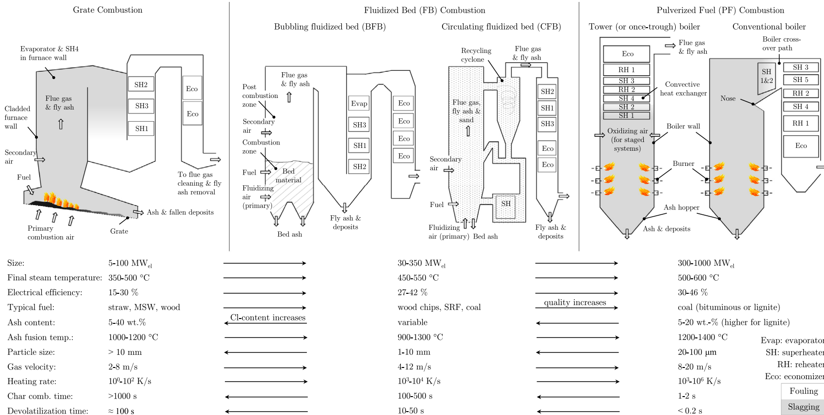
Fig. 1. Combustion systems for solid fuels showing locations threatened by slugging and fouling. Typical process conditions, fuels, steam temperatures and efficiency values are given.
