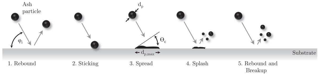
Fig. 58. Particle impaction on a solid substrate: possible phenomena.
