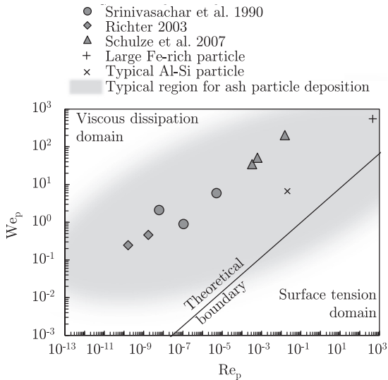
Fig. 95. Particle deposition regime map showing that energy losses due to viscous deformation are dominating ash deposition (see Table 19 for properties of the large Fe-rich and Al-Si particle).
