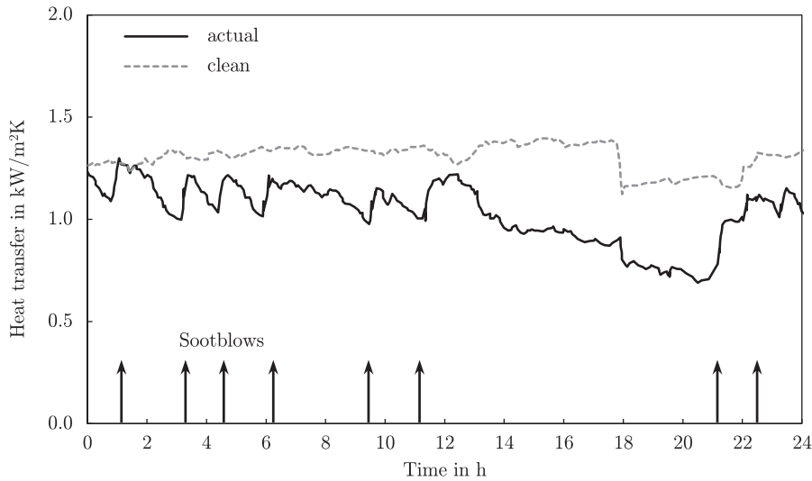
Fig. 31. Heat transfer characteristics over time for a radiant superheater (taken from Wynnyckyj et al. [272]).
