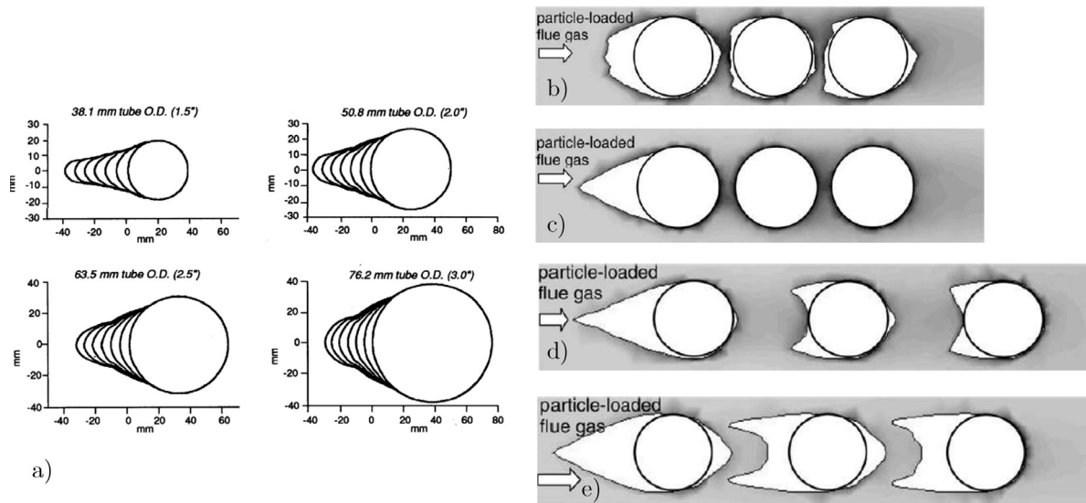
Fig. 35. Deposit built-up over time: (a) predictions from Wagoner and Yan [278] considering inertial impaction for a period of six hours and a gas velocity of 18.3 m/s, and (b) to (e) CFD simulations of Tomczek and Wactawiak [253] considering inertial impaction and condensation. Fig. (b) show predictions for a platen superheater after 9 month operation and d_p = 1 \mu\text{m} ; Fig. (c) platen superheater after 5 month operation and d_p = 33 \mu\text{m} ; Fig. (d) and (e) show platen superheater with wider longitudinal pitch after 9 month and d_p = 33 and 50 \mu\text{m} , respectively.
