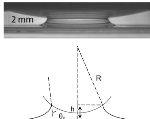
Fig. 52. Photograph and capillary bridge between a spherical particle and a liquid (taken from Yuan and Lee [347], originally from Restagno et al. [352]; reprinted with permission. Copyright 2009 American Chemical Society).
