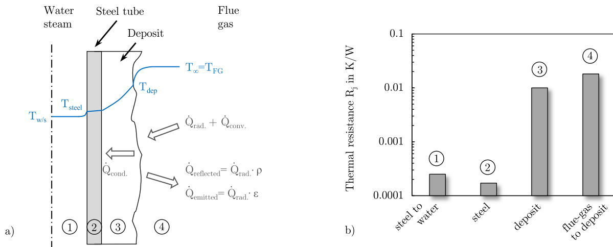
Fig. 33. Effect of deposit on heat transfer: (a) heat transfer to and through ash deposits (modified from Zbogar et al. [273]) and (b) calculated thermal resistances for a flat wall analogous to Eq. (38) with A_o = 1 \text{ m}^2 .
