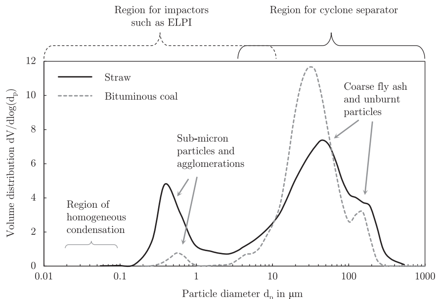
Fig. 15. Typical ash particle size distribution from PF combustion of straw and bituminous coal. Taken from tests in an entrained flow reactor [175,188].
