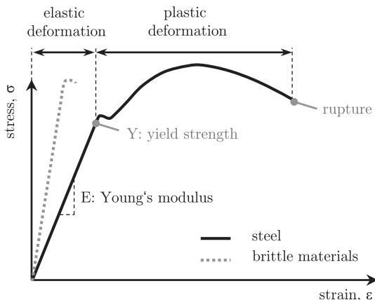
Fig. 40. Yield-stress diagram for steel and brittle material.
