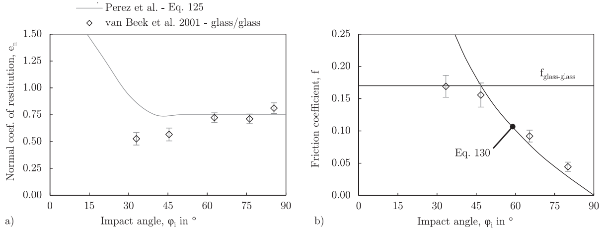
Fig. 82. Results from glass particle impactation on flat solid glass surface (taken from van Beek et al. [268]): (a) normal coefficient of restitution as a function of impact angle \varphi_i , and (b) friction coefficient f as a function of impact angle \varphi_i for a glass/glass material combination.
