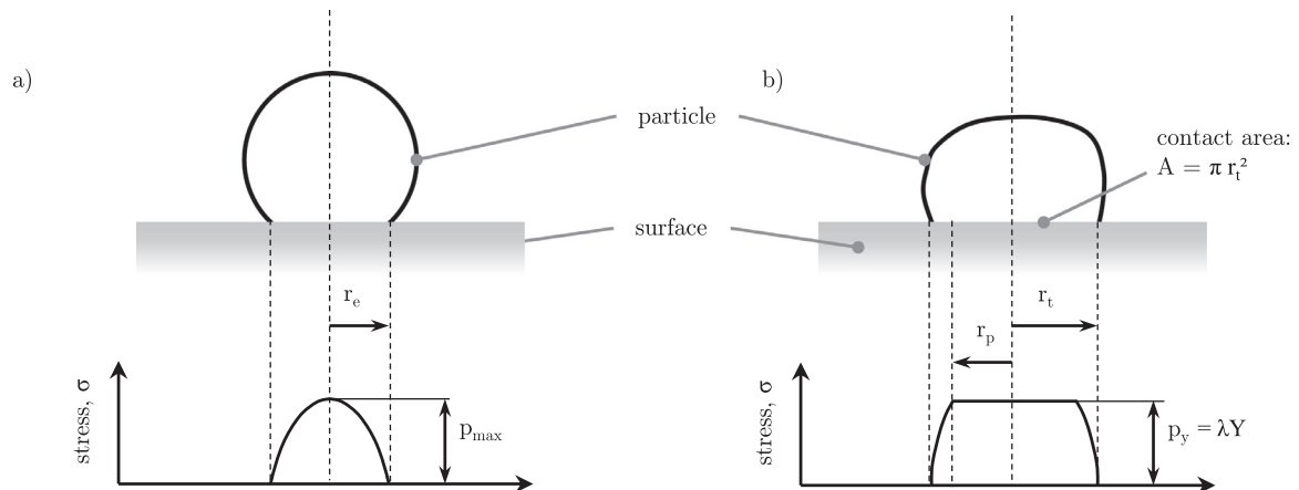
Fig. 77. Pressure distribution for an impacting particle: (a) for a pure elastic contact with Hertz distribution and (b) for an elastic-plastic contact (figure adopted and modified from [267,301,511]).
