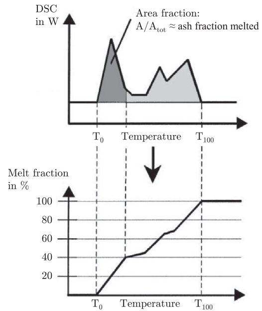
Fig. 42. Calculation of a melting curve from STA data (adopted from Hansen et al. [87]).
