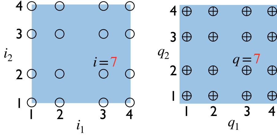
(a) Nodes of cubic Lagrange element (b) Gaussian quadrature points
