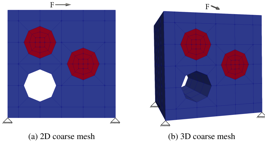
Figure 3: Discretization of the heterogeneous material at the coarsest mesh level and the prescribed boundary conditions.
