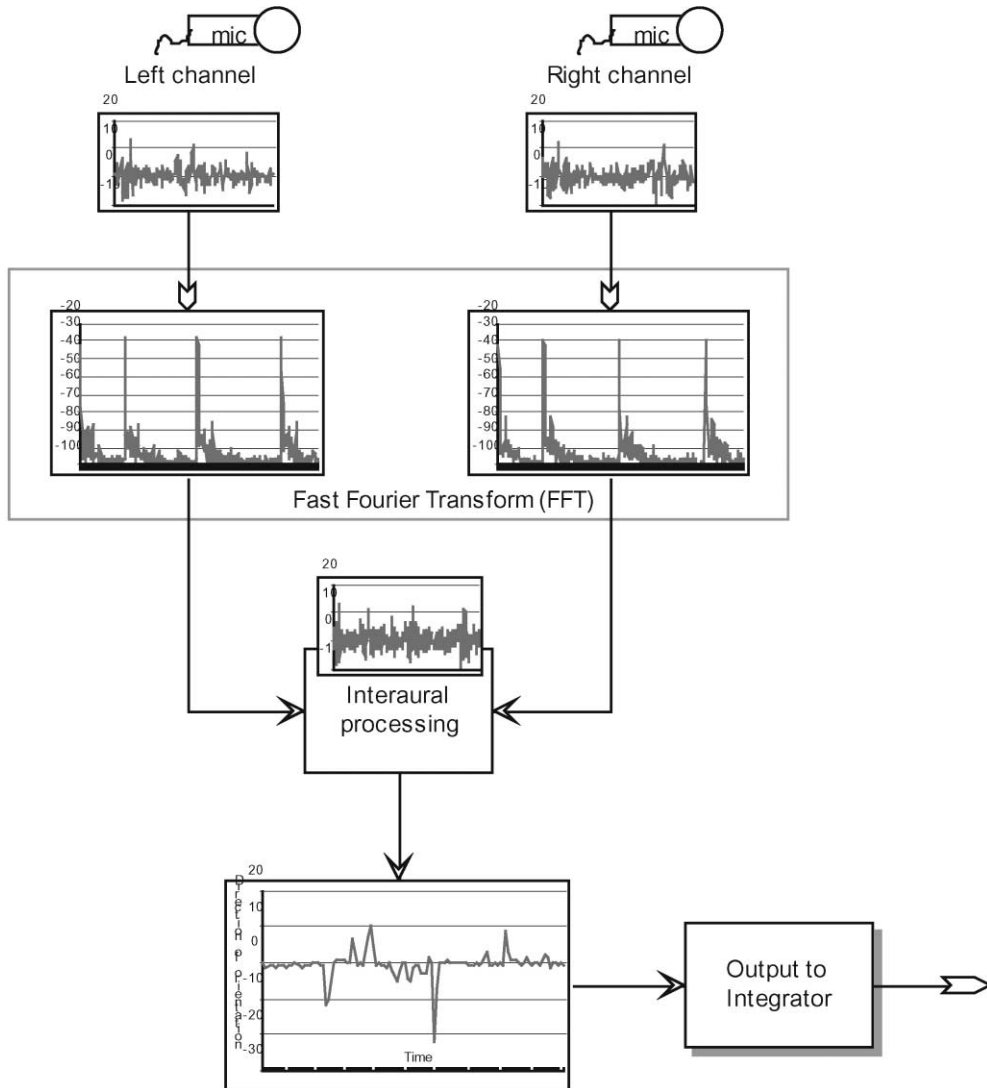
Fig. 8. Auditory processing: stages of the auditory processing performed by our system is shown. First, simultaneous sampling of the left and right channels is made. An FFT is then performed on each channel. The difference between the two channels are then used as the output for spatial hearing response.
