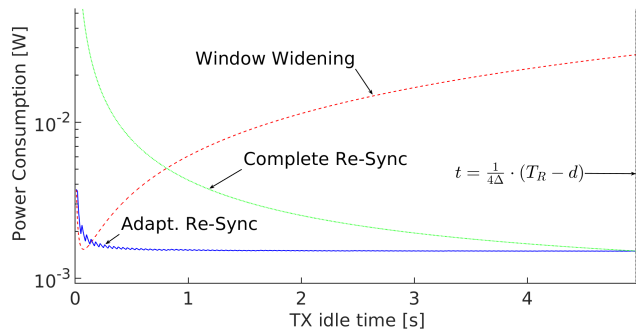
Figure 4: Joint power consumption for reception and transmission for different strategies with T_R = 10 ms.
