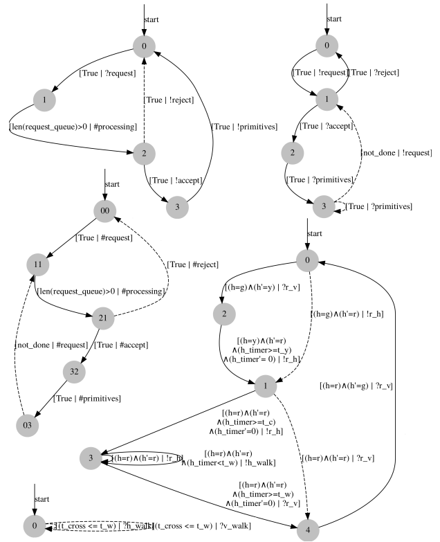
Fig. 3. Reading from left to right, then top to bottom: \mathcal{C}_{scheduler} , \mathcal{C}_{car} , \mathcal{C}_{scheduler} \otimes \mathcal{C}_{car} , \mathcal{C}_{horizontal\_lights} , \mathcal{C}_{pedestrian} .
