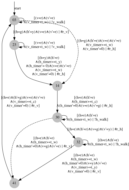
Fig. 4. \mathcal{E}_{lights} = \mathcal{E}_{horizontal\_lights} \otimes \mathcal{E}_{vertical\_lights}
