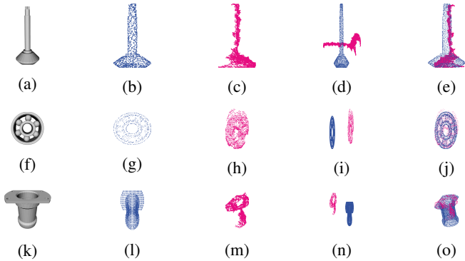
Fig. 6: The first column shows the CAD models of the gearbox components tree, bearing, and pipe. The second one shows the mesh sampled point cloud from the CAD model for each component. The cluster extracted from the point cloud scene (Fig. 1b) is shown in column three. Column four shows the initial source and target point cloud. The alignment results of GPIS-S2SPR are shown in the last column.
