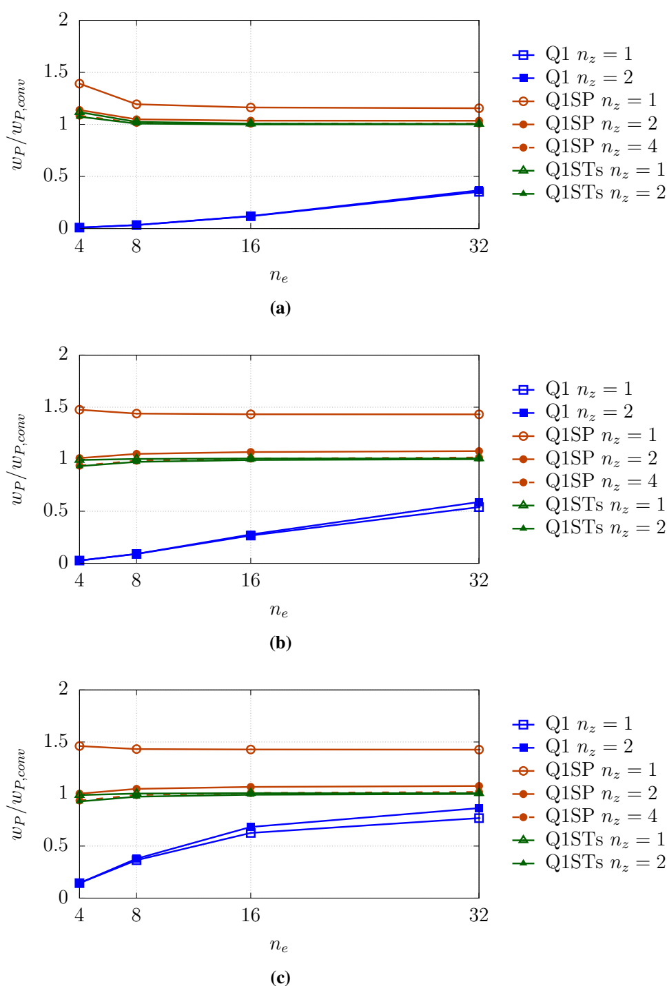
Fig. 21 Deflection at the central point of the thick plate for different number of elements ( n_e ) in planar directions. a a/h = 100 , b a/h = 50 and c a/h = 20
