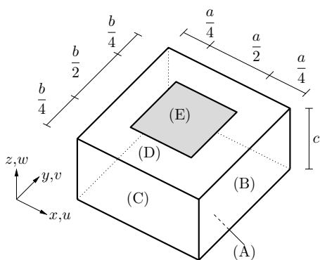
Fig. 34 Geometry of the 3D benchmark problem
