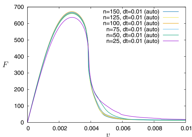
Fig. 39 Displacement-reaction force curve for different plane discretizations
