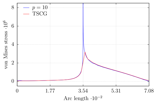
Fig. 15 Von Mises stress along diagonal from point P to point A on top face for the isotropic trunk space of order p = 10 on a 8 \times 8 \times 8 mesh, geometrically graded towards the traction boundary and for a 64 \times 64 \times 64 mesh of TSCG elements
