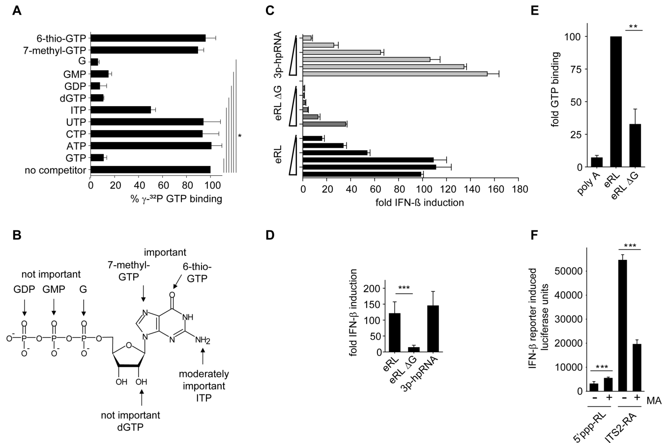
Figure 6. The eRL functions as an aptamer and binds GTP. (A) Competitive binding studies with IVT-eRL, \gamma - ^{32} P GTP and indicated unlabeled competitors. Percentage \gamma - ^{32} P GTP binding = [(amount of radiolabeled GTP bound in the presence of unlabeled competitor) / (amount of radiolabeled GTP bound in the absence of indicated competitor)] \times 100. Graph combines two independent experiments each in duplicates (four measurements per data point \pm S.D.), * P < 0.05 . (B) Data from competitive binding experiments mapped to the structure of GTP. (C, D) HEK293-RIG-I-IFN- \beta reporter cells were stimulated with eRL, eRL \Delta G or 3p-hpRNA at 0.25; 0.063, 0.016, 0.0039 or 0.00098 \mu g/ml. Luciferase activity was measured 12 h after ligand stimulation. (C) One representative experiment is shown and (D) a statistical analysis at the concentration of 0.063 \mu g/ml combining three independent experiments each in biological duplicates (6 measurements per data point \pm S.D.) is depicted, *** P < 0.001 . (E) GTP binding studies utilizing 0,1 nmol eRL, eRL \Delta G or poly A and \gamma - ^{32} P GTP. GTP binding by eRL is set to 100. Graph combines three independent experiments each in duplicates (six measurements per data point \pm S.D.), * P < 0.05 . (F) Stimulation of HEK293-RIG-I-IFN- \beta reporter cells that were mock-treated or pre-incubated with 10 \mu M mycophenolic acid (MA) for 24 h and subsequently incubated with 0.5 \mu g/ml 5'ppp-RL or 1 \mu g/ml ITS2-RA. Luciferase activity was measured 12 h after ligand stimulation. One individual experiment is shown (first panel) and a diagram combining three independent experiments each in triplicates with data adjusted to the ratio of IFN- \beta activation without and with MA treatment (last panel; nine measurements per data point \pm S.D.), *** P < 0.001 .
