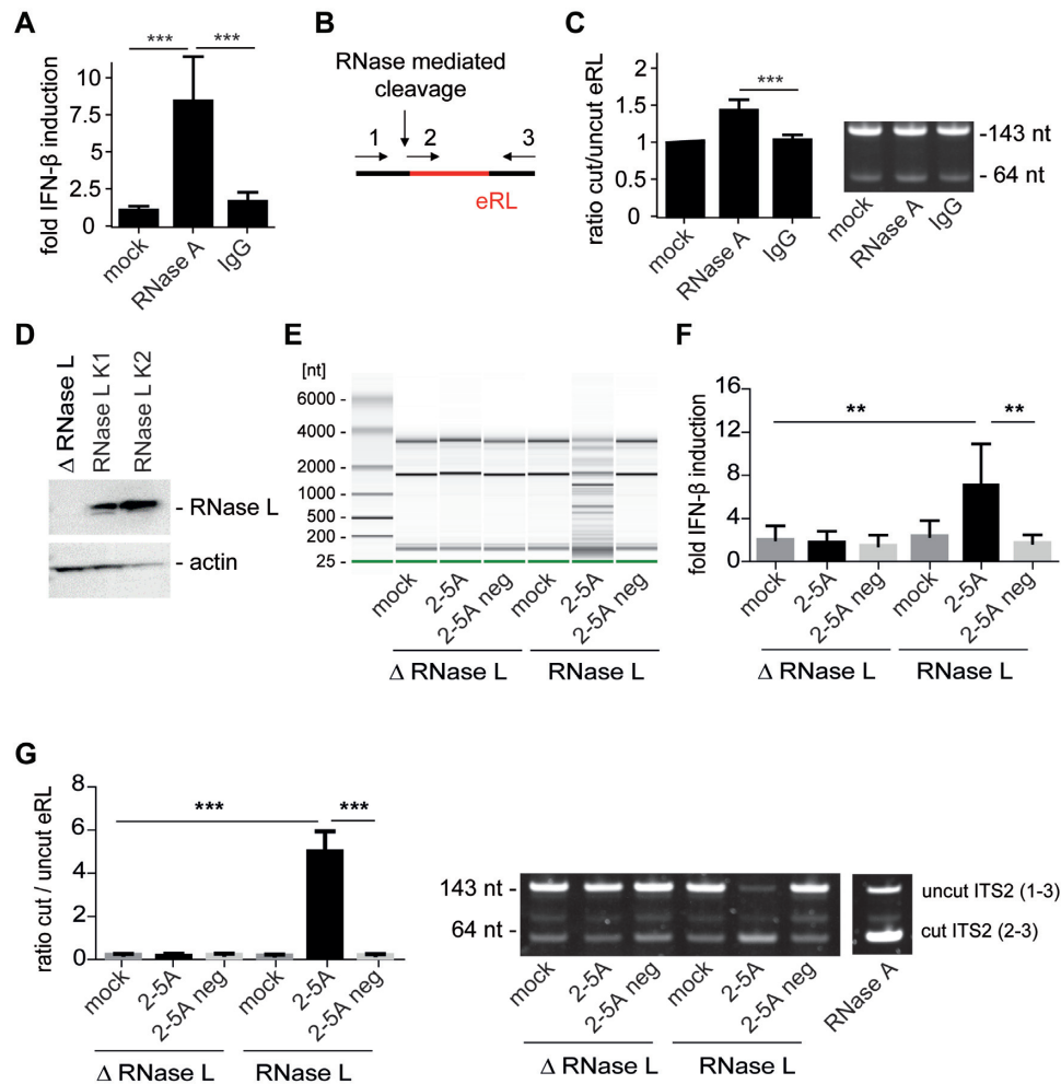
Figure 4. The eRL is generated intracellularly and induces immune activation. (A) HEK293-RIG-I-IFN- \beta reporter cells were mock-treated or transfected with 3.5 \mu\text{g/ml} RNase A and 3.5 \mu\text{g/ml} murine IgG using SAINT-Protein transfection reagent and interferon reporter activity was measured 24 h after transfection. Graph combines three independent experiments each in biological quadruplicates (12 measurements per data point \pm S.D.), *** P < 0.001 . (B) Schematic illustration of the RT-PCR strategy using three primers (depicted as 1, 2 and 3, see Materials and Methods) in one reaction to analyze uncut or cut ITS2 fragments (eRL). (C) Cleavage of eRL was determined in qRT-PCR after 24 h. Left panel combines three independent experiments each in technical duplicates (six measurements per data point \pm S.D.). *** P < 0.001 . Right panel depicts a representative fragment analysis in a 12% PAA gel stained with SYBRGold. One individual experiment of three independent experiments is shown. (D) Western blot of HEK293-RIG-I-IFN- \beta reporter cells devoid of or reconstituted with RNase L. \beta -actin served as loading control. (E) RNase L-deficient ( \Delta RNase L) and RNase L-competent (RNase L K2) HEK cell lysates were untreated (mock) or incubated with 2'-5'-oligoadenylate (2-5A) containing lysate or control lysate (2-5A neg). After incubation of 1 h at 37°C, RNA was purified and RNA integrity investigated utilizing Pico RNA chips on an Agilent bioanalyzer. One individual representative experiment of three independent experiments is shown. (F) RNAs depicted in (E) were transfected into HEK293-RIG-I-IFN- \beta reporter cells at 5 \mu\text{g/ml} RNA each. Fold IFN- \beta induction was determined after 12–16 h. Graph combines three independent experiments each in biological duplicates (6 measurements per data point \pm S.D.), ** P < 0.01 . (G) RNAs depicted in (E) were analyzed for generation of eRL by RT-PCR. Left panel combines three independent experiments each in technical duplicates (six measurements per data point \pm S.D.), *** P < 0.001 . Right panel depicts a representative fragment analysis in a 12% PAA gel stained with SYBRGold. One individual experiment of three independent experiments is shown. In vitro RNase A-digested HEK293 RNA served as positive control.
