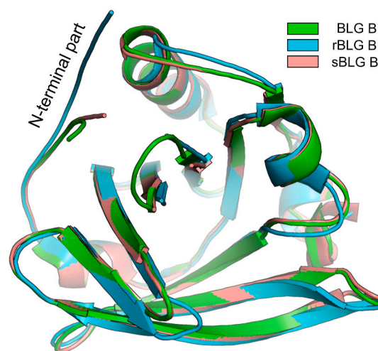
Fig. 1. Superposition (C \alpha ) of lactoglobulin crystal structures: BLG B (PDB ID: 3NPO), rBLG B (PDB ID: 5K06) and sBLG B (PDB ID: 6QI6). The overall structure of all compared variants is almost the same but N-terminal part of the variant with additional N-terminal methionine (cyan) has different conformation than observed in natural protein isoform B (green) or a variant with N-terminal mutations L1A/I2S (pink). (For interpretation of the references to colour in this figure legend, the reader is referred to the Web version of this article.)
