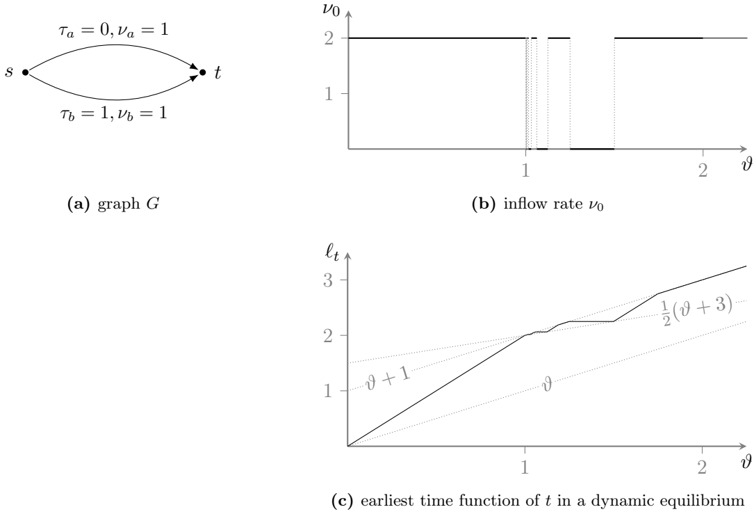
Figure 4.6: Example with nonright-monotone inflow rate for which the \alpha -extension does not work.
