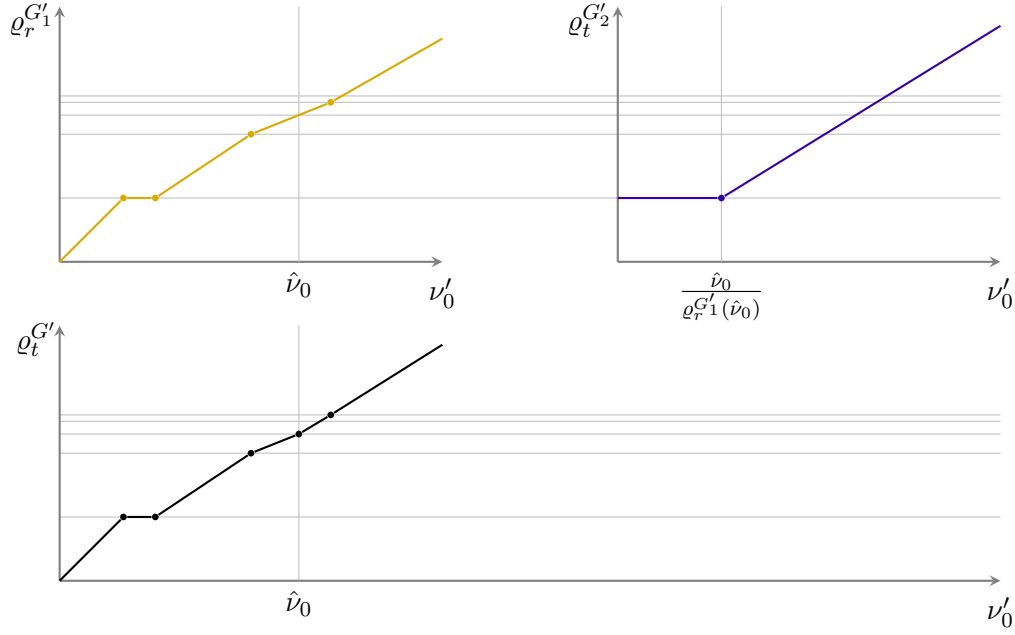
Figure 4.7: Series composition G' = G'_1 * G'_2 at common vertex r . The breakpoint of \varrho_t^{G'} at \hat{\nu}_0 results from the breakpoint of \varrho_t^{G'_2} .
