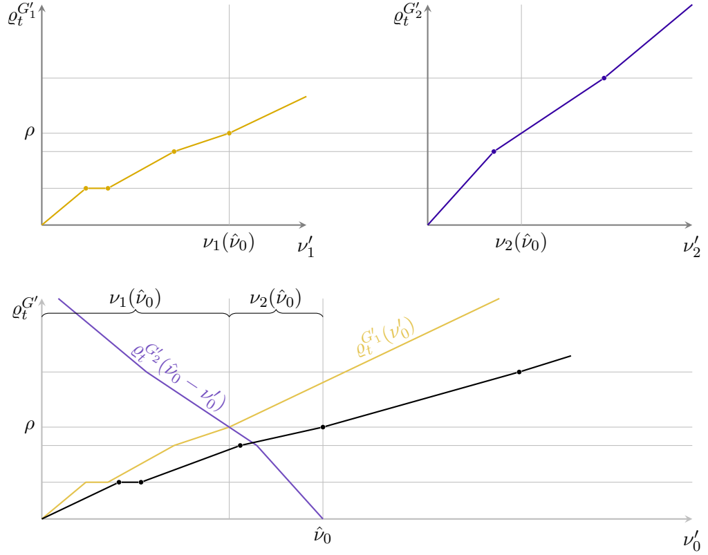
Figure 4.8: Parallel composition G' = G'_1 \parallel G'_2 . The breakpoint \hat{\nu}_0 of \varrho_t^{G'} is based on the intersection of \varrho_t^{G'_1}(\nu'_0) and \varrho_t^{G'_2}(\hat{\nu}_0 - \nu'_0) at a breakpoint of \varrho_t^{G'_1} .
