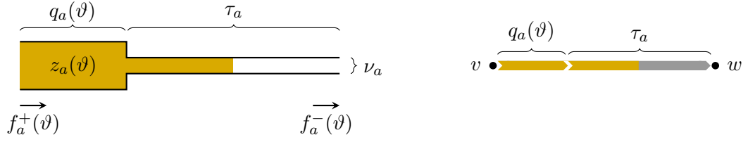
Figure 4.1: A link (left) represented by an arc a = (v, w) \in A with transit time \tau_a , capacity \nu_a , inflow rate f_a^+ , outflow rate f_a^- , queue length z_a , and queuing delay q_a . We use a simplified representation (right).
