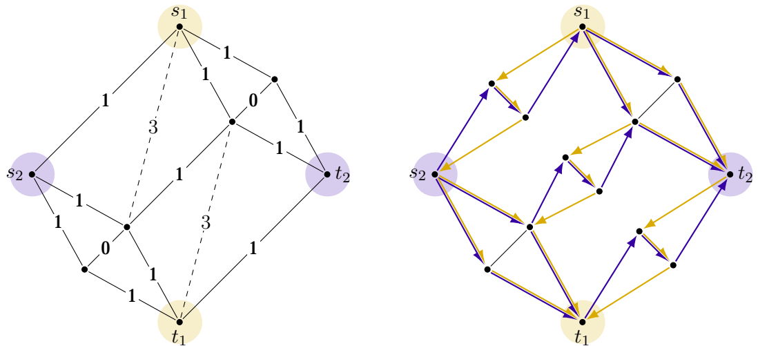
(a) An undirected graph with annotated edge lengths. The shortest path networks E_1 and E_2 agree (solid edges).
