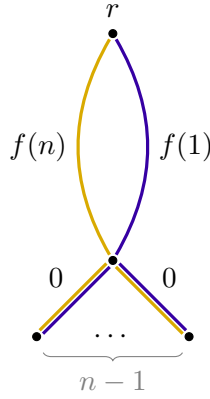
Figure 5.8: A broadcast game with root r which exhibits a large price of anarchy. The edges are annotated with their cost c_e . The social optimum (yellow) and a Nash equilibrium of large social cost (violet) are highlighted.
