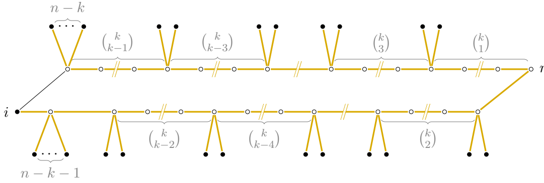
Figure 5.7: The deviation of player i from the highlighted strategy profile in this multicast game leads to a small decrease of the potential. Vertices with associated players are represented by filled nodes ( \bullet ). All total edge costs are constant and one.
