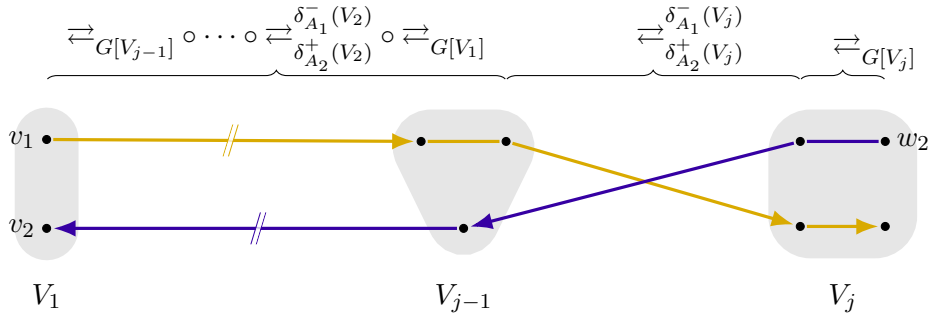
Figure 3.7: In the j -th iteration of Line 5 in Algorithm 2 , the relation \rightleftharpoons is extended by concatenating previously computed paths with arcs from the disjoint sets \delta_{A_1}^-(V_j) and \delta_{A_2}^+(V_j) , and arc/edge-disjoint paths in G[V_j] . The path for the first component is extended by appending to its end. The path for the second component is extended by prepending to its beginning.
