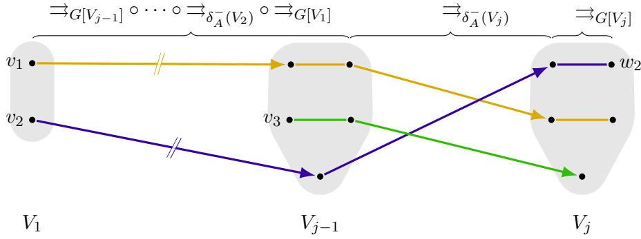
Figure 3.4: In iteration j of Algorithm 1 , the relation \Rightarrow is extended by concatenating previously computed paths with pairwise different arcs from \delta_A^-(V_j) and edge-disjoint paths in G[V_j] .
