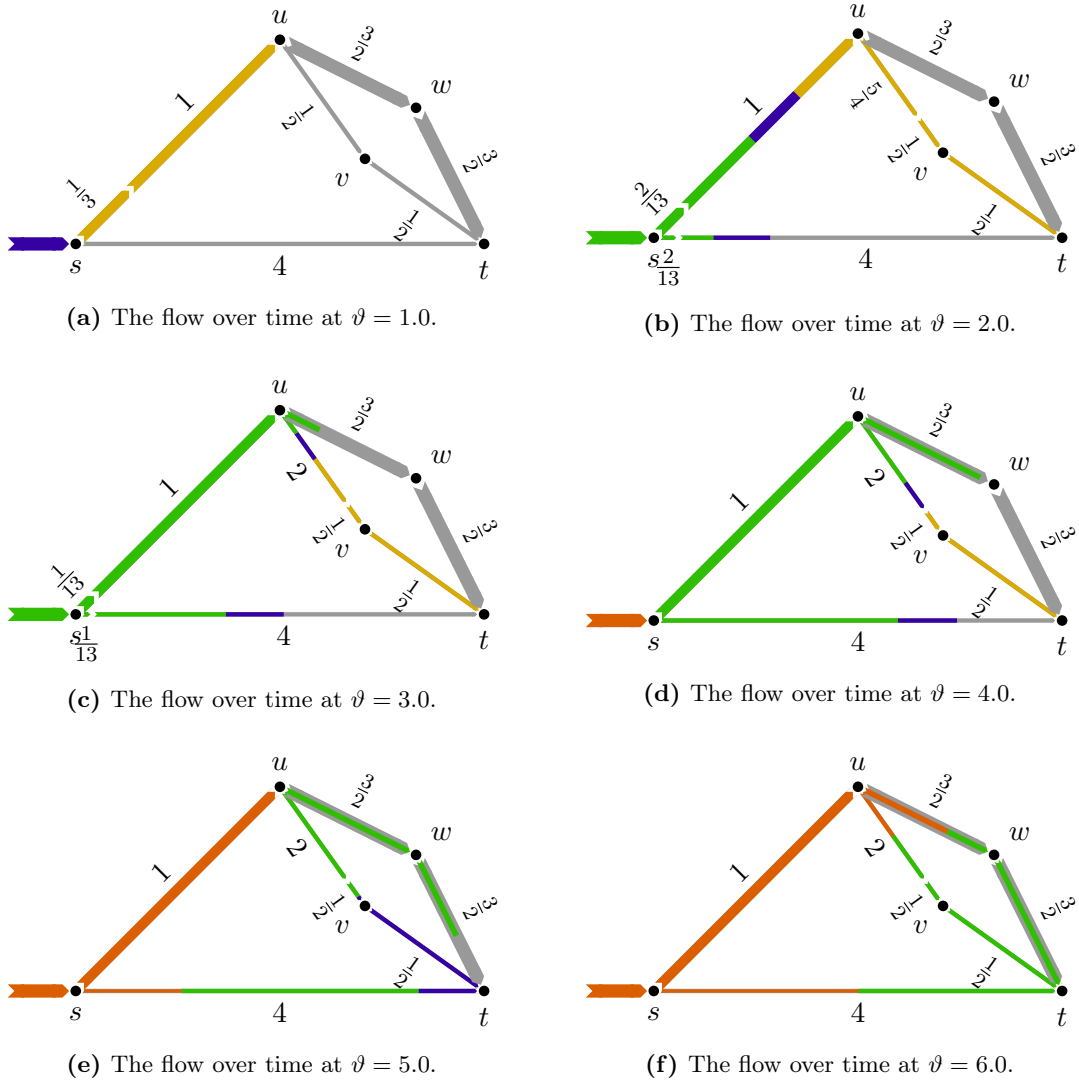
Figure 4.4: A dynamic equilibrium in the network depicted in Figure 4.2. The flow is colored with respect to its phases. Within each phase, the flow pattern is the same. Every arc a is annotated with its respective queuing delay q_a(\vartheta) (if it is nonzero) and its transit time \tau_a . The relative contribution of q_a(\vartheta) to the total transit time q_a(\vartheta) + \tau_a is indicated by a small white gap in the link.
