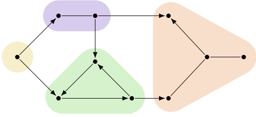
(a) A mixed graph and a partition of its vertices.
