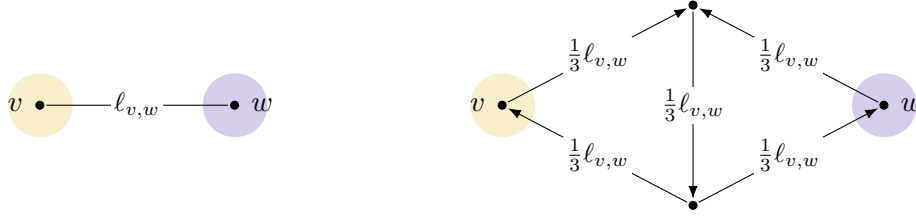
Figure 3.5: The gadget (right) for resolving the ambiguity in the orientation of an edge (left).
