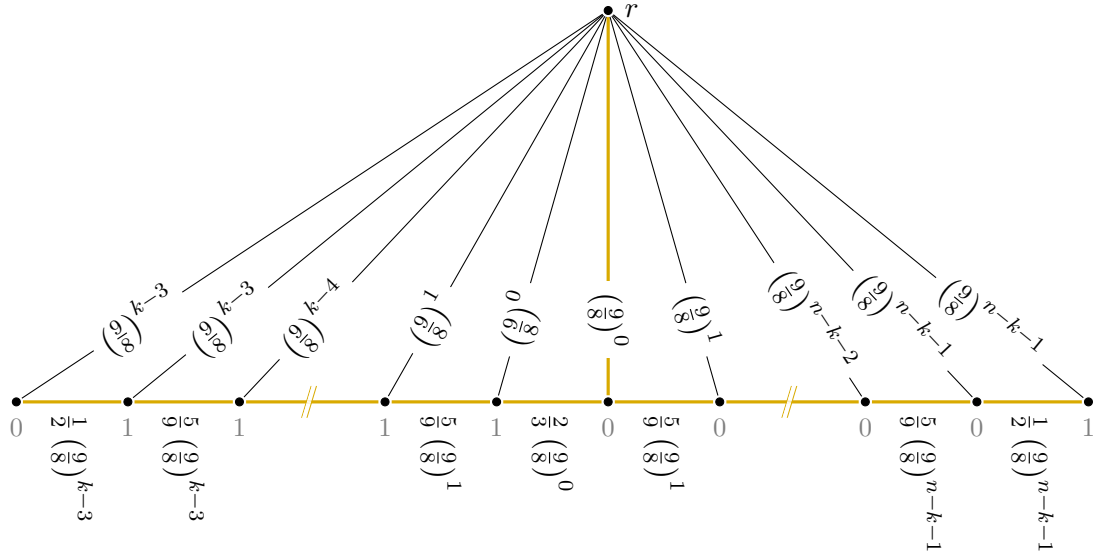
Figure 5.16: The edge cost c^{(z)} in the fan with z_i = 1 for 1 < i < k and z_i = 0 for k \leq i < n . The vertices i \in [n] are annotated with their value of z_i in gray. T_k is highlighted in yellow.
