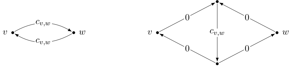
Figure 5.3: Two opposite arcs (left) are replaced by a gadget (right). The arcs are annotated with their cost.
