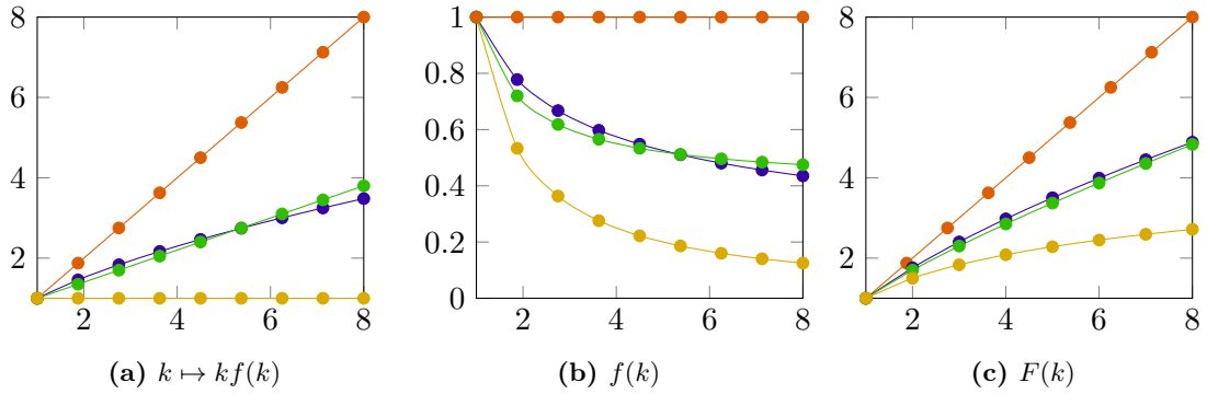
Figure 5.1: The relevant cost functions under constant total edge cost (yellow), polynomial total edge cost with \alpha = 0.6 (violet), affine total edge cost with s = 0.4 (green), and linear total edge cost (red).
