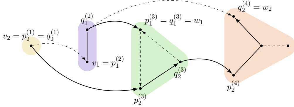
(c) The decomposition of two disjoint paths by intermediate vertices based on the graph's partition.
