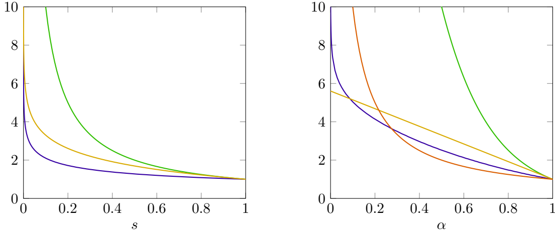
(a) The two bounds 1 - \ln(s) (yellow) and 1 + W_0((1-s)/(es)) (violet) on the price of stability under affine total cost. The bound of 1/s on the price of anarchy (green) is included for comparison.
