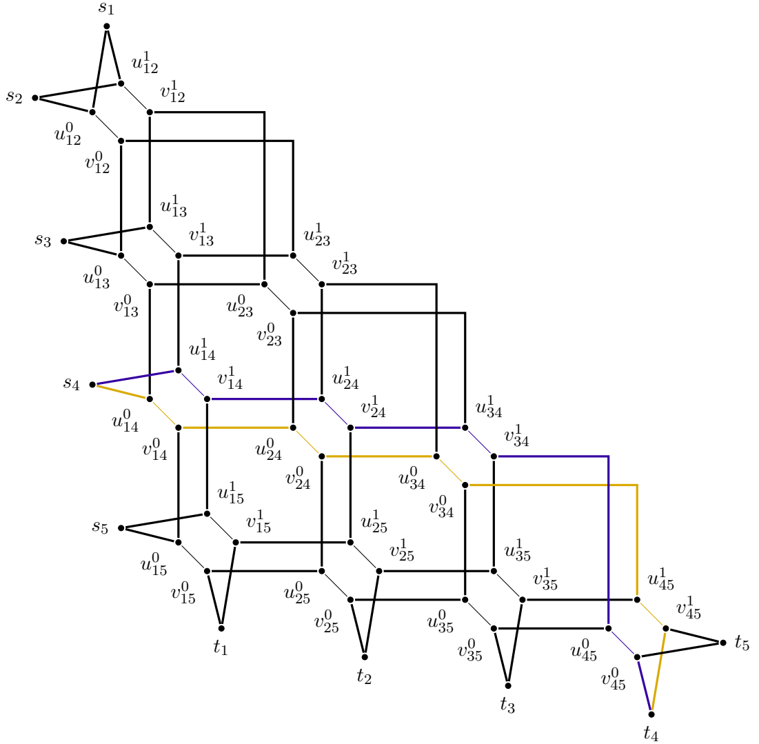
Figure 5.4: An instance resulting from an intermediate cost-sharing game with n = 5 players. Thick connections represent paths of length L . Thin edges correspond to the resources of the intermediate game. The two highlighted paths are the dominant strategies of player 4, which correspond to her strategies in the intermediate game.
