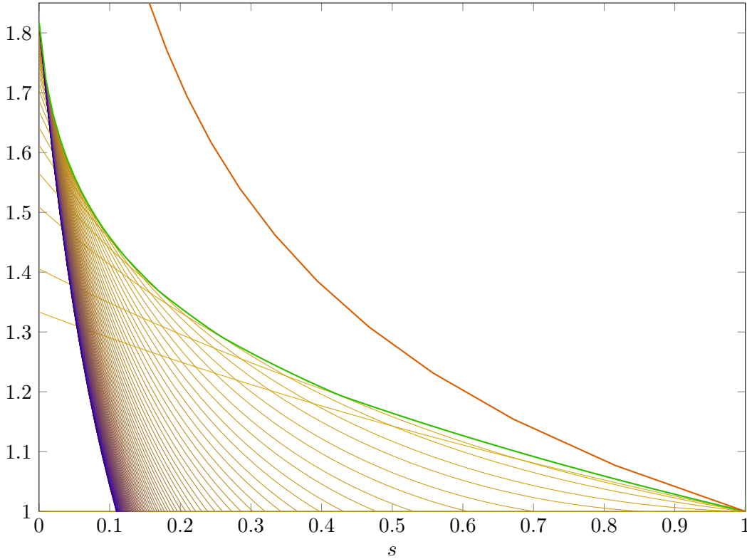
Figure 5.18: Lower bounds to the price of stability for a ne total edge cost. The bounds \text{PoS}(G_n, c^{(z_{\lceil n/2 \rceil})} \mid S_n, T_{\lceil n/2 \rceil}) are plotted for n = 1 (yellow) to n = 100 (violet). The bound resulting from maximizing over all n \in \mathbb{N} is highlighted in green. The upper bound based on Theorem 5.23 is plotted in red.
