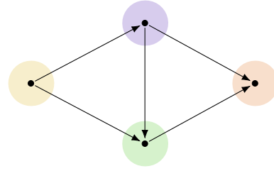
(b) The directed acyclic graph resulting from contracting the partition.
