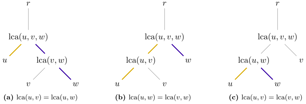
Figure 5.13: The contributions of paths in S to c'_\sigma(\sigma_u \setminus \sigma_w) - c_\sigma(\sigma_w \setminus \sigma_u) . Paths highlighted in yellow add to c'_\sigma(\sigma_u \setminus \sigma_w) . Paths highlighted in violet add to c_\sigma(\sigma_w \setminus \sigma_u) .
