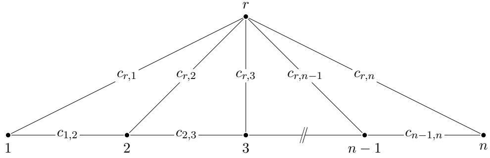
Figure 5.15: The fan graph with n players.
