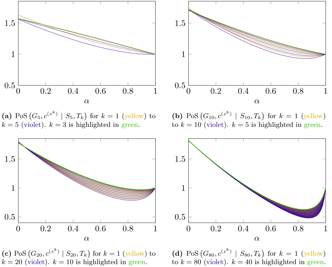
Figure 5.19: The dependency of PoS ( G_n, c^{(z^k)} \mid S_n, T_k ) on k \in [n] for polynomial total edge cost.
