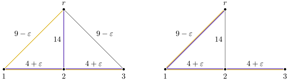
Figure 5.2: Braess's paradox for the price of stability in an instance with f(k) = 1/k (left). The social optima and Nash equilibria are highlighted in yellow and violet, respectively. The deletion of \{r, 3\} decreases the price of stability from (22 + 2\varepsilon)/(17 + \varepsilon) to 1 (right).
