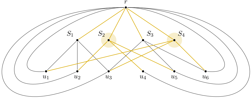
Figure 5.5: The broadcast game resulting from an exact 3-set cover problem with universe U = \{u_1, \dots, u_6\} and family of subsets \mathcal{S} = \{S_1, \dots, S_4\} . The strategy profile supported by the highlighted edges corresponds to the exact covering \{S_2, S_4\} .
