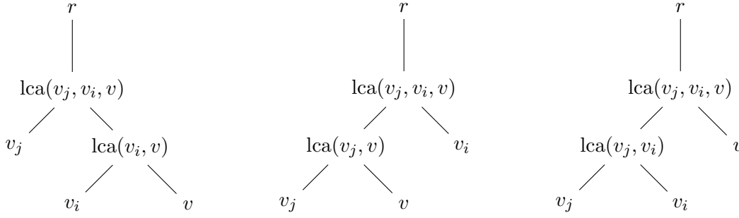
Figure 5.12: Possible relationships between the lowest common ancestors in S .
