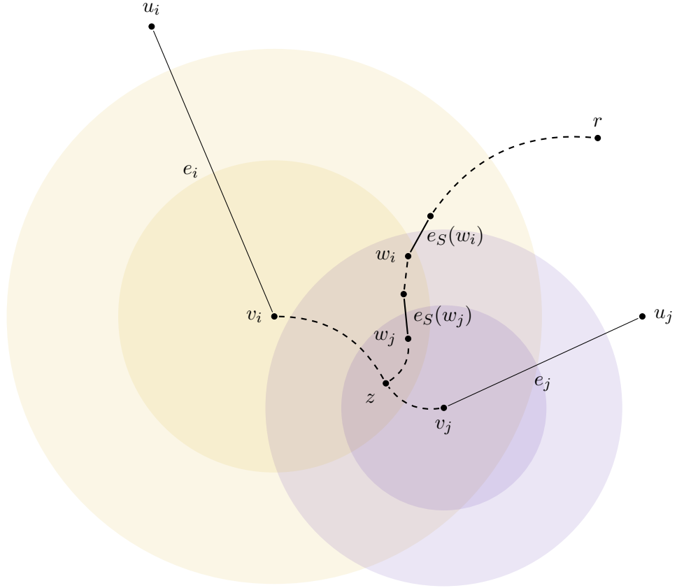
Figure 5.14: Charging scheme from the proof of Theorem 5.33 . The yellow circles represent the absorption radius \alpha c_{e_i} f(1) and the charging radius \rho \alpha c_{e_i} f(1) around v_i with respect to d_{T, \bar{f}} . Similarly, the violet circles represent the absorption radius \alpha c_{e_j} f(1) and the charging radius \rho \alpha c_{e_j} f(1) around v_j with respect to d_{T, \bar{f}} . The thick connections represent edges and paths in T . The vertex z is on both paths, T[v_i, w_j] and T[v_j, w_j] .
