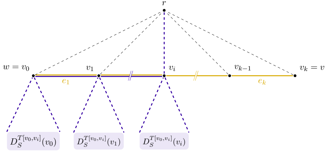
Figure 5.11: The strategy \sigma^{w-T \rightarrow v_i} as considered in the proof of Lemma 5.30. The descendants of T[w, v_i] use the path T[w, v] (yellow) to follow v_i (violet).
