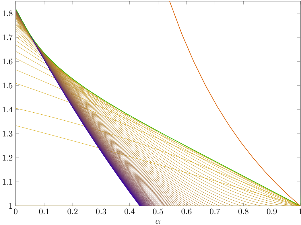
Figure 5.20: Lower bounds to the price of stability for polynomial total edge cost. The bounds \text{PoS}(G_n, c^{(z_{\lceil n/2 \rceil})} \mid S_n, T_{\lceil n/2 \rceil}) are plotted for n = 1 (yellow) to n = 100 (violet). The bound resulting from maximizing over all n \in N is highlighted in green. The upper bound based on Theorem 5.24 is plotted in red.
