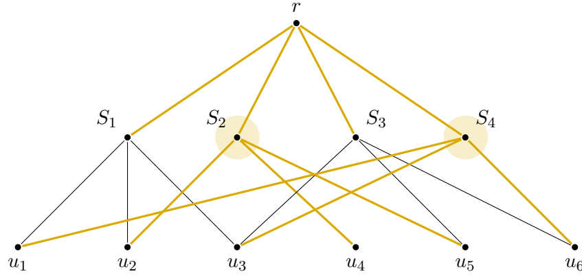
Figure 5.6: Illustration of the reduction for the hardness of global potential minimization. The depicted broadcast game is based on an exact 3-set cover instance with universe U = \{u_1, \dots, u_6\} and the family of subsets \mathcal{S} = \{S_1, \dots, S_4\} . The highlighted edges support a strategy profile that corresponds to the exact set covering \{S_2, S_4\} .
