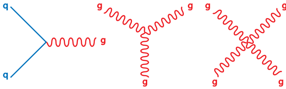
Figure 1. Fundamental quark and gluon interactions of QCD
