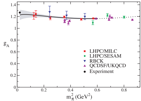
Figure 10. World's collection of lattice QCD results for g_A [2, 5, 6, 7]
