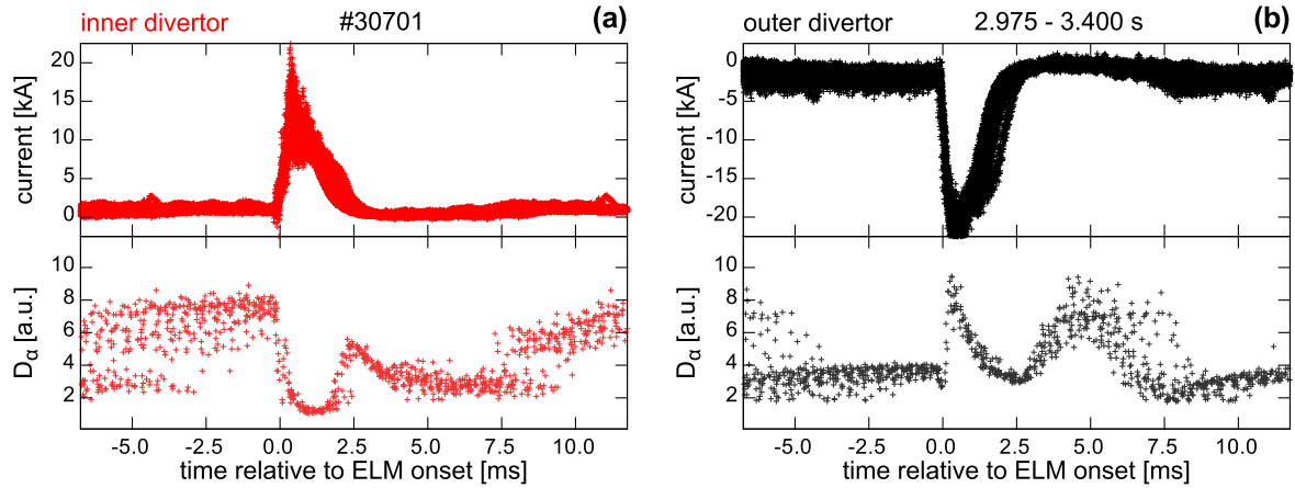
Figure 4. ELM synchronised evolution of the SOL current and D_\alpha emission at the (a) inner and at the (b) outer divertor target: the SOL current flows from the outer to the inner target. The D_\alpha emission at the outer target increases approximately 2.5 ms after ELM onset a second time, which is not connected to another ELM crash but to high neutral recycling.
