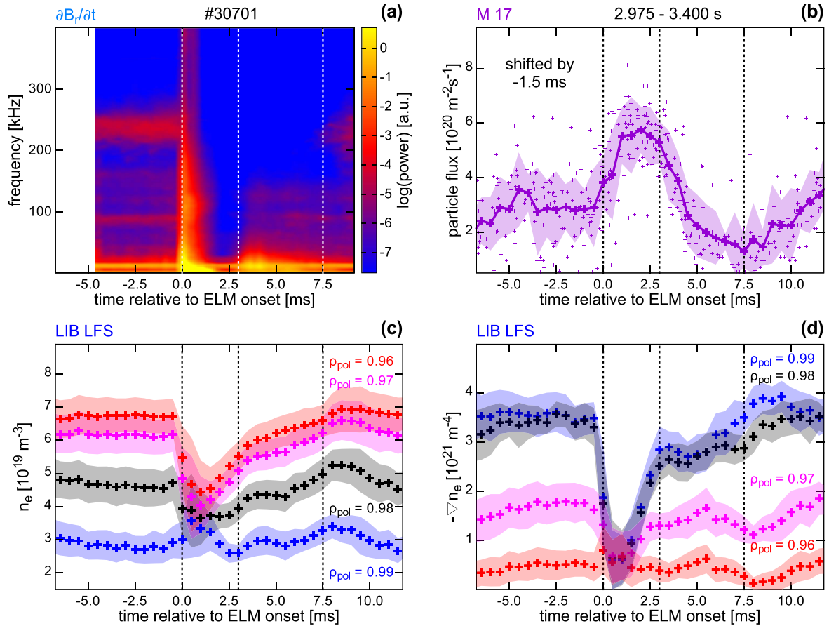
Figure 9. Correlating the ELM synchronised n_e pedestal recovery with the magnetic activity and the main chamber neutral fluxes: (a) ELM synchronised frequency histogram of \partial B_r / \partial t measured at the LFS midplane, (b) LFS midplane neutral fluxes (shifted by -1.5 ms), (c) n_e and (d) \nabla n_e at four radial positions ( \rho_{\text{pol}} ) in the confined plasma from the pedestal top (0.96) to the steep gradient region (0.99). During the recovery of \nabla n_e in the steep gradient region (between 1.5 and 3.0 ms) a phase of low magnetic activity is found. During this period also the neutral particle flux in the main chamber is enhanced, well before the D_\alpha emission and n_e increase in the outer divertor and the appearance of the high recycling regime.
