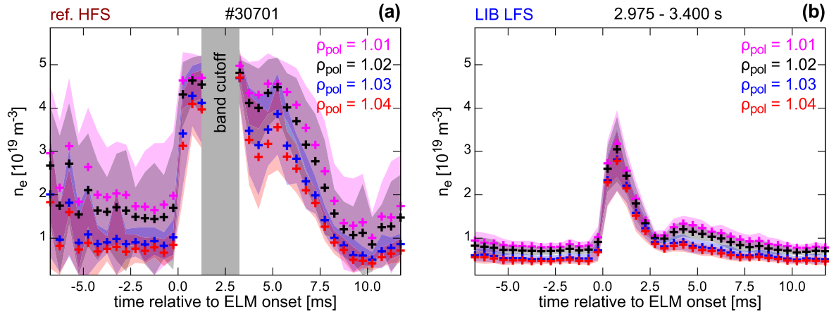
Figure 8. Comparison of the inter-ELM (a) HFS and (b) LFS SOL n_e evolution: n_e at four different radial positions ( \rho_{\text{pol}} ) from near (1.01) to far (1.04) SOL. After the ELM crash a strong asymmetry between LFS and HFS SOL n_e is observed, which timescale corresponds to the appearance of the HFSHD. During this period the SOL density shoulder appears at the LFS.
