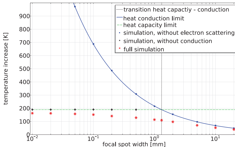
FIGURE 3 Maximum temperature increase at the focal spot in the heat capacity limit (small spot widths) and the heat conduction limit (broad spot widths) as calculated in Monte Carlo simulations and transient FEA. The electron beam had a power of 90 kW and an energy of 300 keV, the target surface velocity was 200 m/s
