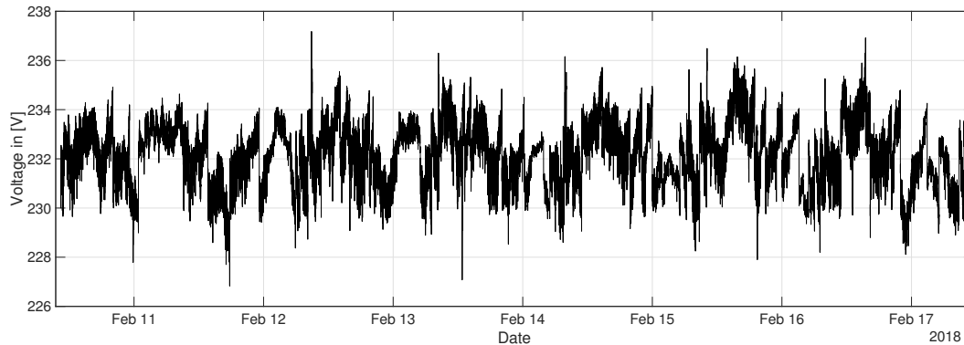
Figure 3.10: One week voltage recording from Munich [own illustration].
