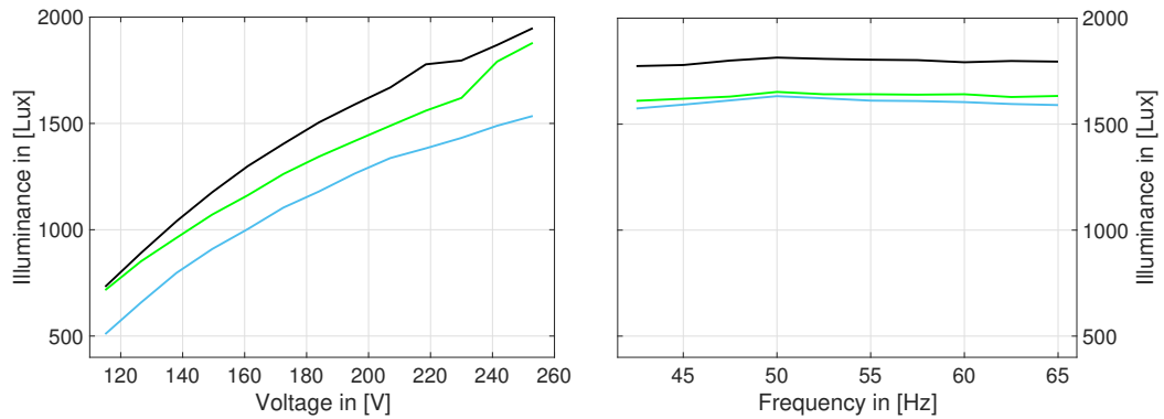
Figure 4.7: Illuminance dependent on voltage (left) and frequency (right) for three samples of CFL lamps.
