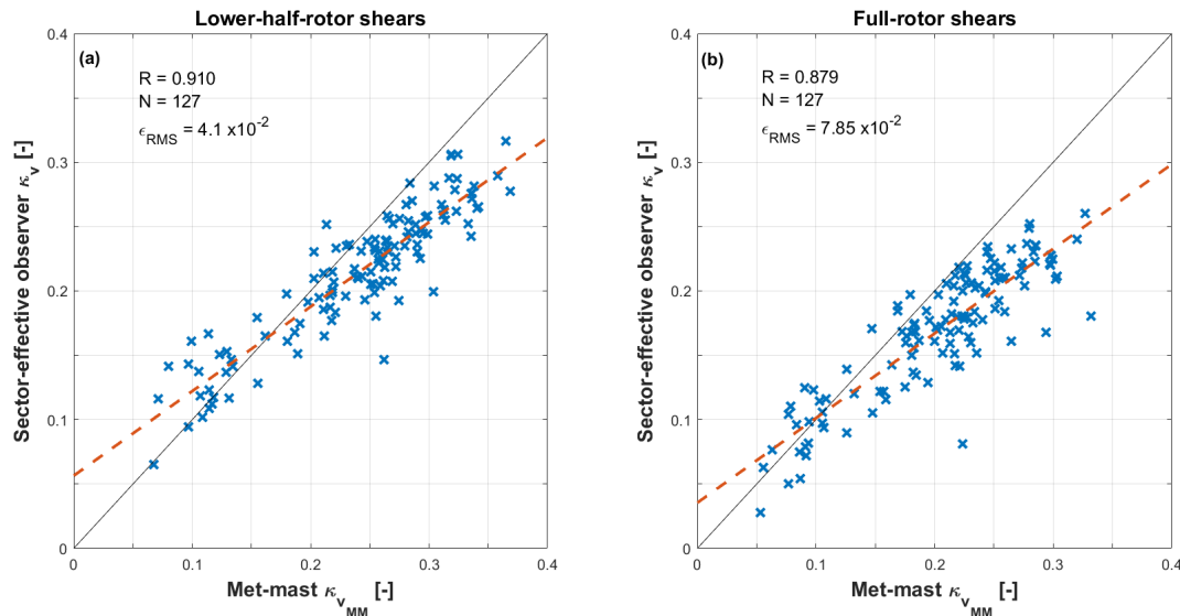
Figure 4. Correlation between 10 min averages of the vertical linear shears measured with the met mast and the sector-effective observer. Lower-half-rotor shears (a); full-rotor shears (b). Dashed red line: linear best fit; dashed black line: ideal match; R : Pearson's correlation coefficient; N : number of data points; \epsilon_{\text{RMS}} : root mean square error.
