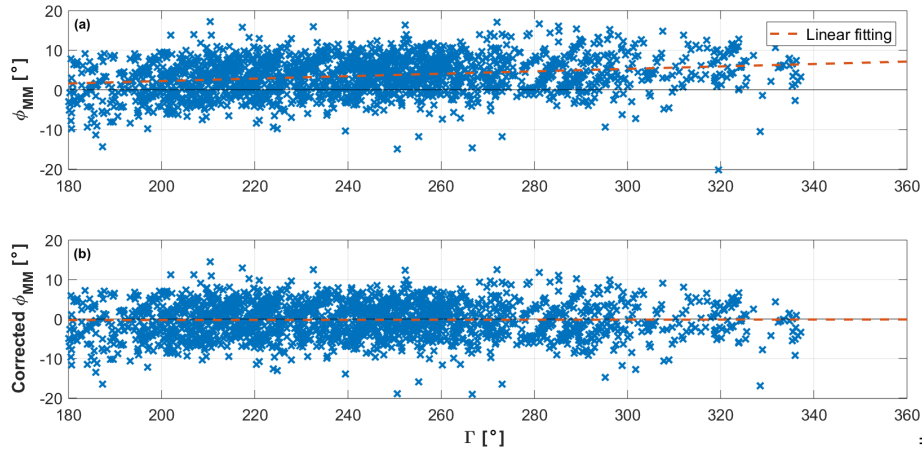
Figure 5. The 10 min averages of met-mast horizontal wind misalignment angle \phi_{MM} vs. wind direction at the met-mast \Gamma before (a) and after (b) correction for yaw encoder error.
