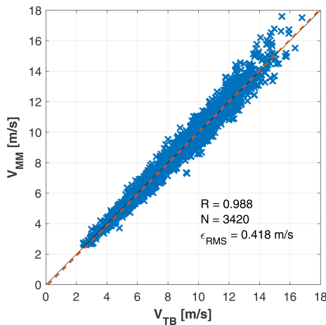
Figure 6. Correlation between 10 min averages of met-mast hub-height wind speed V_{MM} and rotor-effective wind speed V_{TB} estimated with the torque balance equation. Dashed red line: linear best fit; dashed black line: ideal match; R : Pearson’s correlation coefficient; N : number of data points available; \epsilon_{RMS} : root mean square error.
