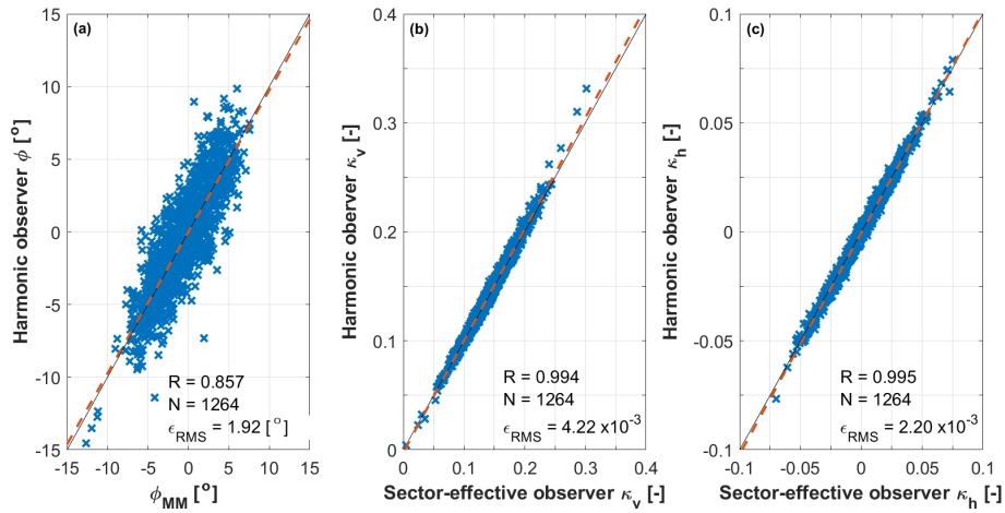
Figure 7. Correlation of 10 min averages between estimated parameters (y axis) and their reference quantities (x axis) for V \geq 8 \text{ m s}^{-1} . Yaw misalignment angle (a); vertical linear shear (b); horizontal linear shear (c). Dashed red line: linear best fit; dashed black line: ideal match; R : Pearson’s correlation coefficient; N : number of data points; \epsilon_{\text{RMS}} : root mean square error.
