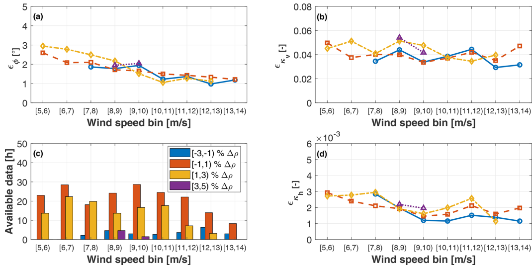
Figure 11. MAE \epsilon vs. binned rotor-effective wind speed for binned density change \Delta\rho with respect to standard air. Yaw misalignment (a); vertical shear (b); hours of available data (c); horizontal shear (d).
