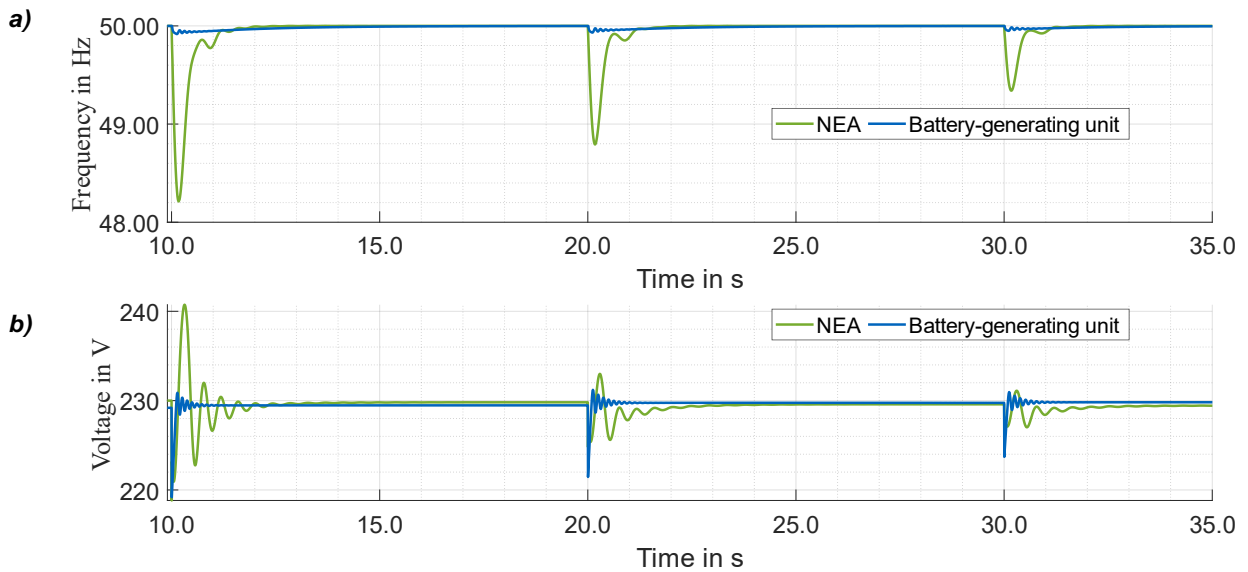
Figure 8: Performance comparison between NEA and battery-generating unit (simulated) for the evaluating load profile
