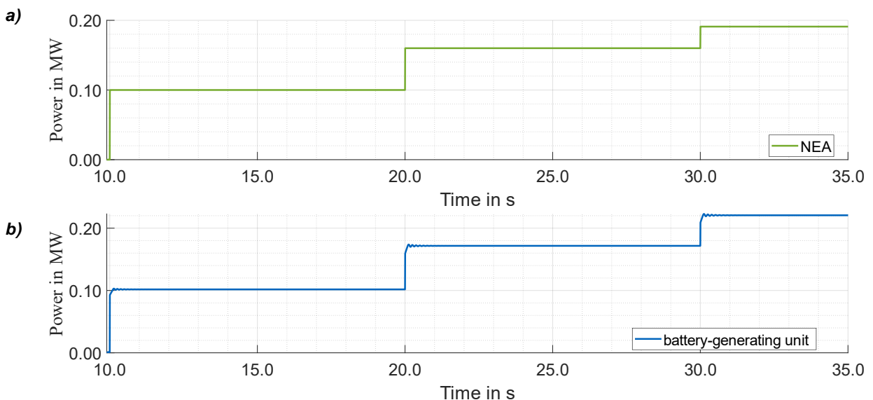
Figure 7: Evaluating load profile according to ISO8528-5 for the a) NEA and b) battery-generating unit
