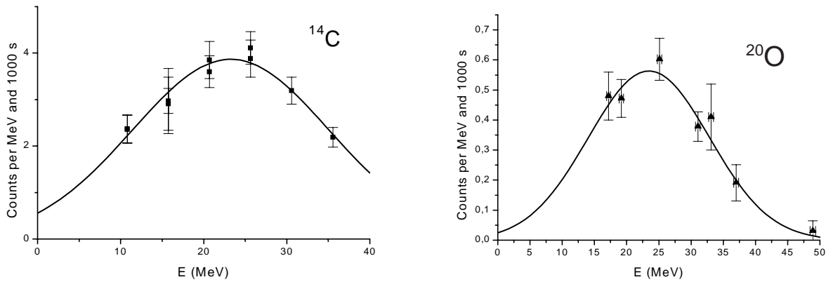
Figure A.4.12.: Kinetic energy distributions of ^{14}\text{C} and ^{20}\text{O} from ^{245}\text{Cm}(n_{\text{th}},f) .
