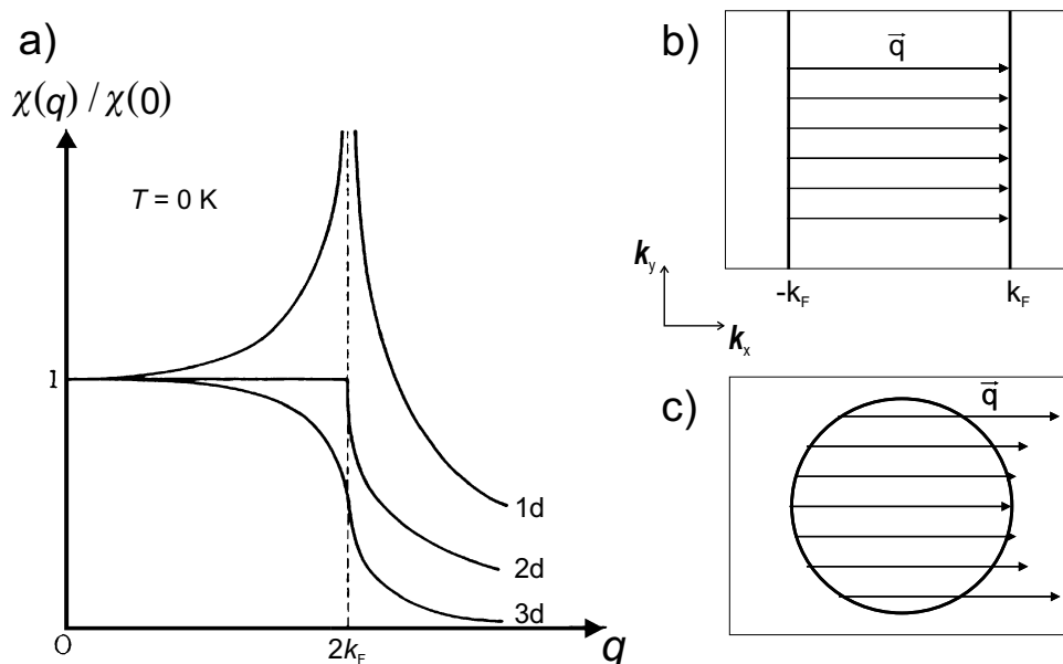
Figure 2.1: a) response function of a free electron gas in an external periodic field V(\mathbf{q}) for different dimensions. b) The Fermi surface of a 1D electron gas consists of sheets at k_x = \pm k_F which can be perfectly nested on each other. c) In a 2D electron system the closed Fermi surface cannot be nested by a single wave vector. Only few electron-hole pairs can be created.
