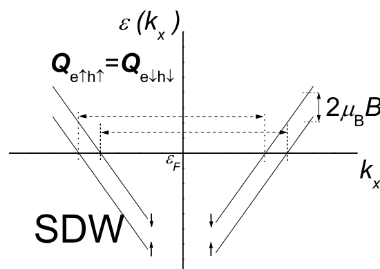
Figure 2.5: Due to the different pairing in SDW systems the nesting vector is unaffected. Therefore, the SDW does not become suppressed in magnetic field.
