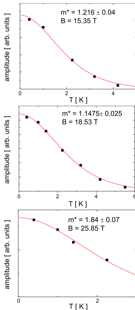
Figure 5.28: Effective mass determination from the temperature dependent amplitude of the dHvA oscillations at 3 different constant fields.
