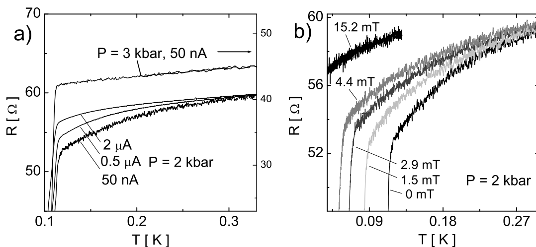
Figure 5.64: Within the CDW state the resistance decrease accelerates already at much higher temperatures than in the NM state ( P = 3 kbar). This decrease strongly depends on the level of the applied current (a) or magnetic field (b).
