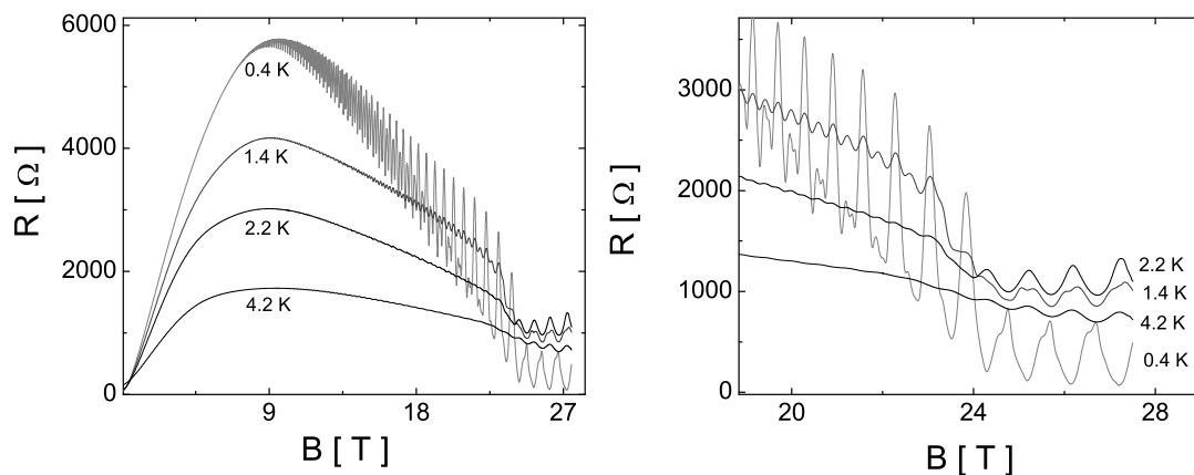
Figure 5.20: Left: several field sweeps at constant T . Right: enlarged high field range. At high fields the background resistance, on cooling, starts to decrease that is accompanied by a phase inversion of the SdH signal.
