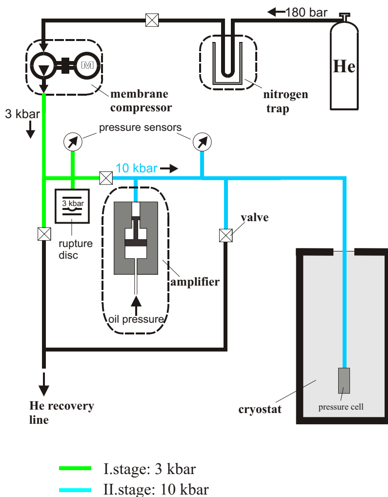
Figure 4.4: Sketch of the ^4\text{He} pressure apparatus.
