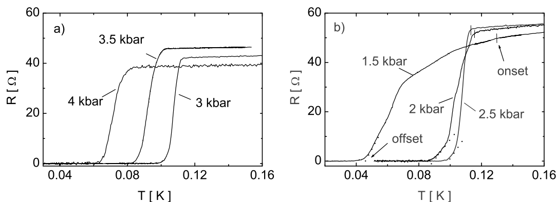
Figure 5.62: Temperature sweeps at different pressures down to the lowest possible temperature. On the left hand side the SC transitions within the NM state are shown. To the right the broadened transitions within the CDW state are plotted. Vertical dashes mark onset temperatures, dotted lines offset temperatures, of the bulk SC transitions.
