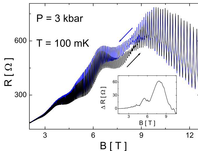
Figure 5.44: Up (black) and down (blue) field sweeps of the magnetoresistance at P = 3 kbar and T = 100 mK. The hysteresis, observed by subtracting one curve from the other, is given in the inset. A clear structure matching the oscillatory features can be seen.
