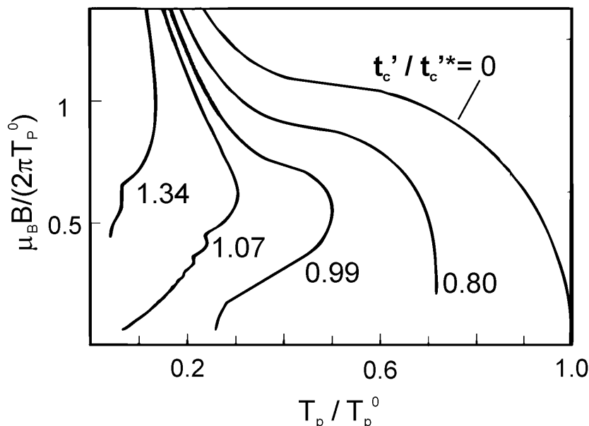
Figure 5.12: Proposed B - T phase lines for a CDW system at different nesting condition. The imperfect nesting is introduced by the effective next-nearest-interchain transfer integral t'_c . t_c'^* corresponds to the value of t'_c for which T_{p,CDW}(B = 0 \text{ T}) = 0 \text{ K} . The kink transition is not shown here.
