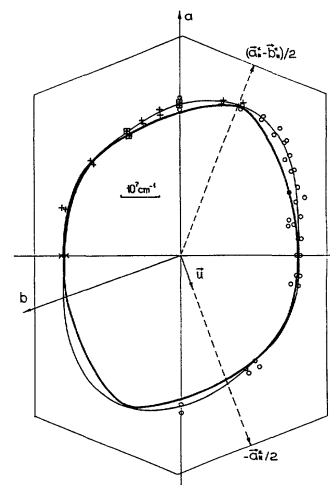
Figure 2.15: Extracted Fermi surface within the a-b plane (thick line) [54].
