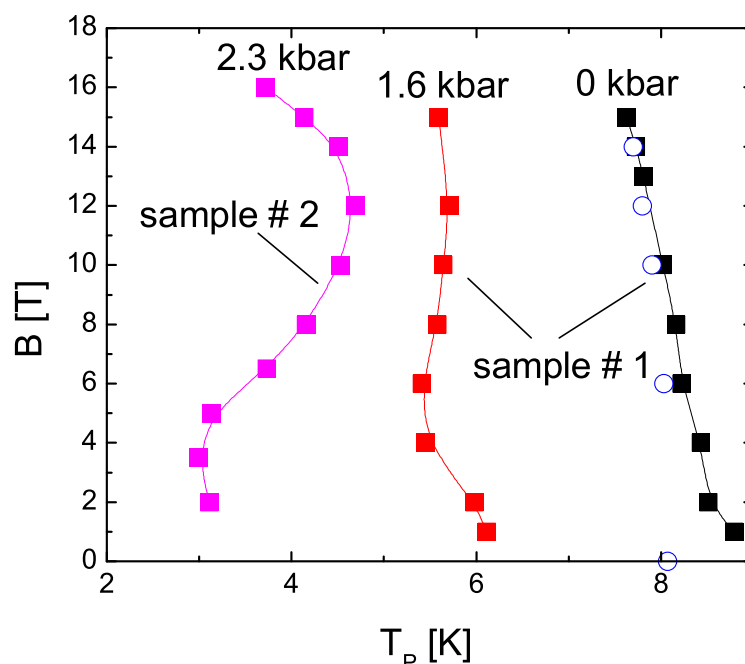
Figure 5.7: Transition temperatures extracted from the Kohler plots for 3 different pressures. At 2.3 kbar the transition temperature clearly increases with field between 5 and 12 T. Open circles mark the transition points found at ambient pressure in specific heat measurements [75]
