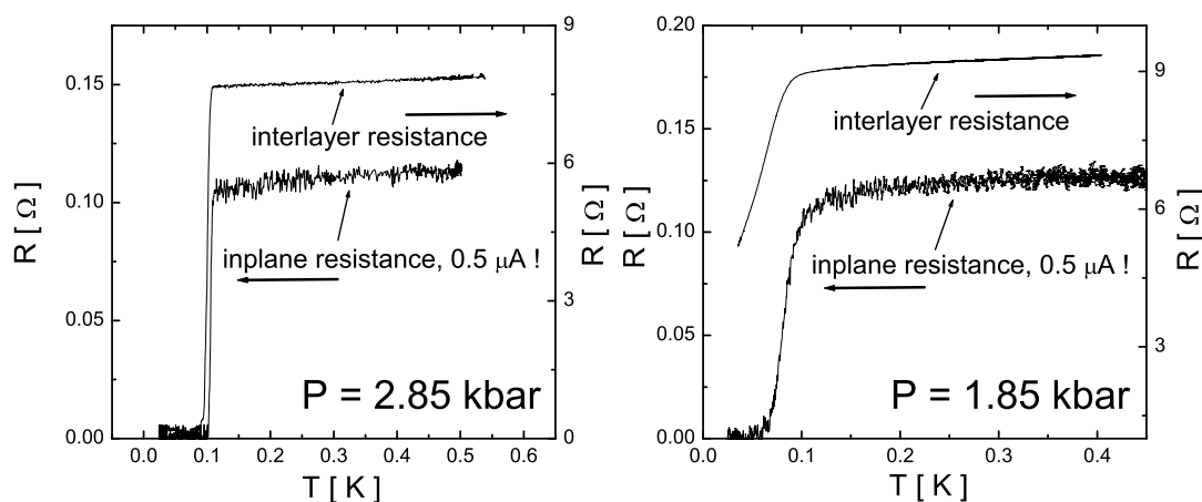
Figure 5.66: Comparison of the in- and interlayer resistance at pressures above (to the left) and below (to the right) the critical value P_0=2.5 kbar.
