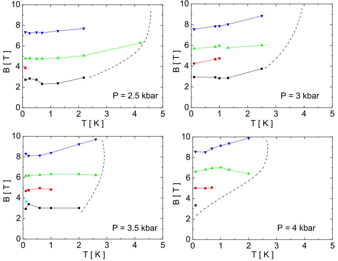
Figure 5.46: FICDW transition points for different pressures. Dashed lines simulate the phase boundaries, the transition points are determined from the maximum curvature of the background resistance of the background resistance
