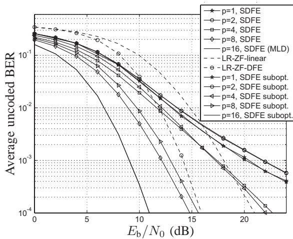
Fig. 4. B = N_R = 8 , ZF detection, QPSK modulation.
