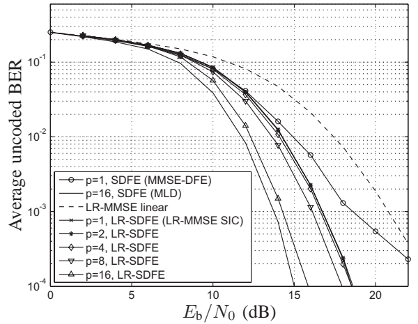
Fig. 5. B = N_R = 8 , MMSE detection, 16-QAM modulation, LR-SDFE uses the suboptimum block Cholesky factorization.
