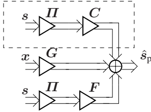
Fig. 2. Equivalent model without the quantizer for SDFE and DFE, with and without the dashed box, respectively.
