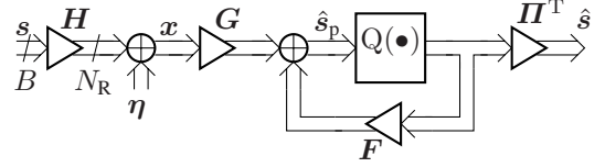
Fig. 1. Decision-feedback equalizer reference model
