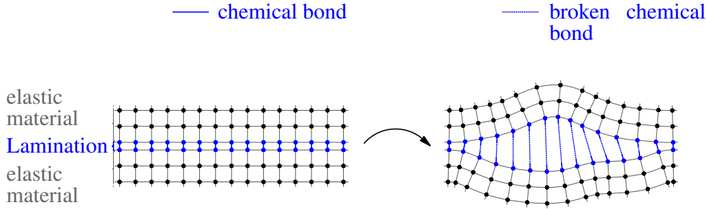
Figure 2.5: Griffith-theory based fracture model
