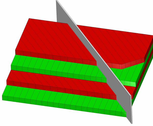
Figure 4.19: A crack in \Omega nonparallel to the beam layers in \mathcal{D}_3
