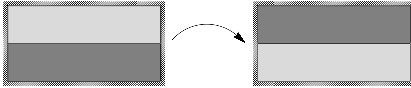
Figure 2.8: Rigid body motion exchanging the position of two bodies, which are enclosed in a rigid environment
