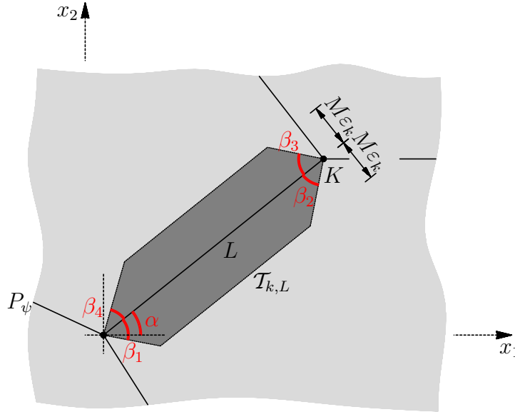
Figure 4.5: The trapezoidal environment \mathcal{T}_{k,L}
