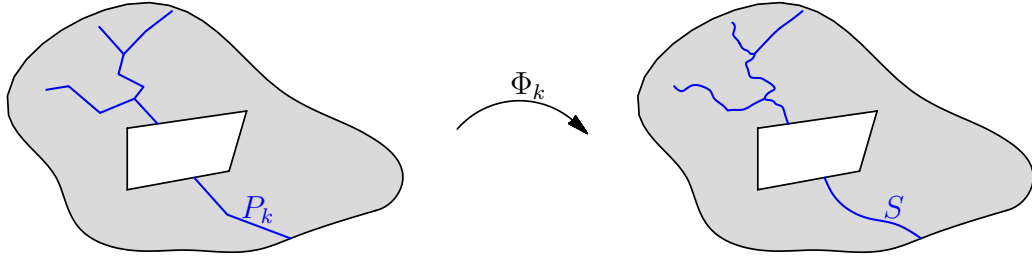
Figure 4.3: A pre-deformation \Phi_k , pulling a piecewise C^1 -hypersurface back onto a polyhedral set
