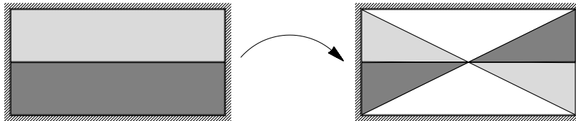
Figure 2.9: An a.e.-injective deformation showing self-intersection
