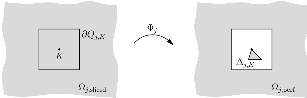
Figure 4.10: The sets \Omega_{j,\text{sliced}} and \Omega_{j,\text{perf}} around K \in \mathcal{K}(P)
