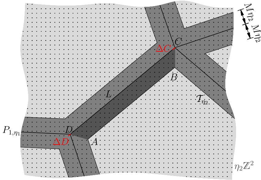
Figure 4.14: The mapping \Psi_{2,\eta_2} on \mathcal{T}_{\eta_2}
