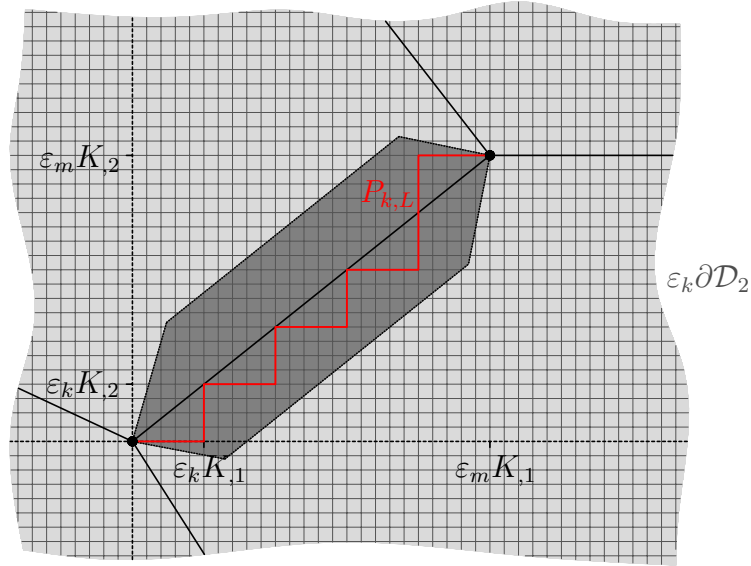
Figure 4.6: The Polygon P_{k,L}
