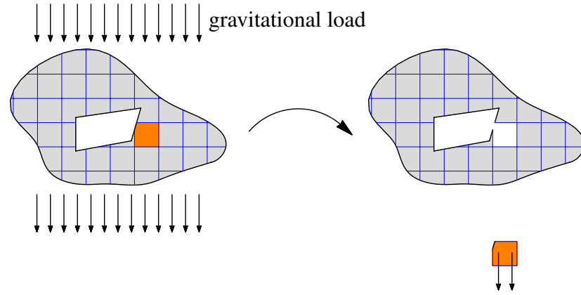
Figure 2.10: No minimum of the total energy in absence of a confinement condition
