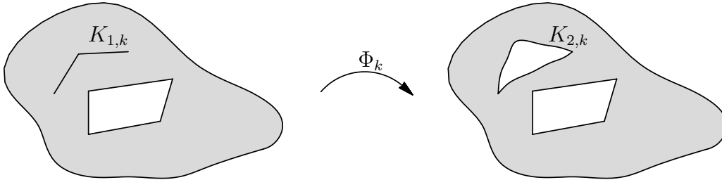
Figure 4.4: A pre-deformation \Phi_k that “slices” \Omega
