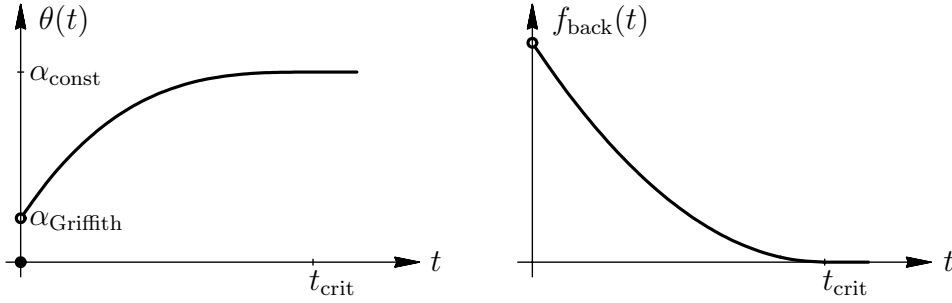
Figure 2.6: \theta as in example 2.2 (left) and its derivative f_{\text{back}} = \frac{d\theta}{dt} (right)
