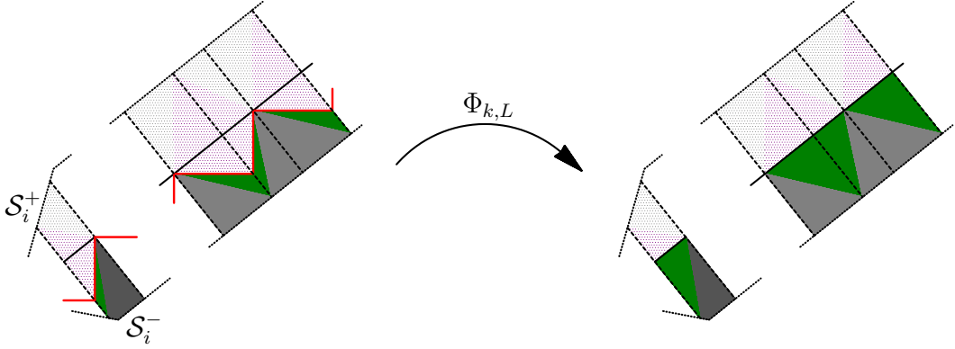
Figure 4.8: Constructing \Phi_{k,L} on each S_i^\pm
