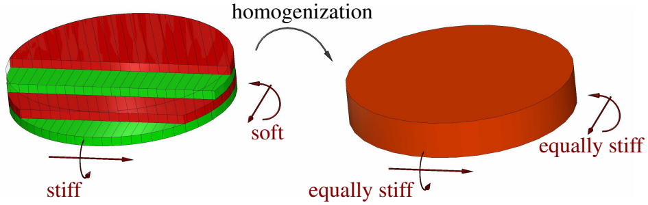
Figure 4.20: Nonzero cord-angle: Bending-isotropy through homogenization
