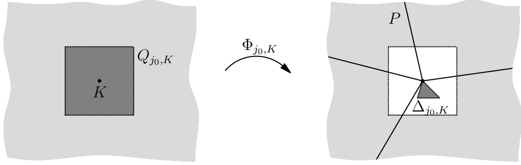
Figure 4.9: The mapping \Phi_{j_0, K}
