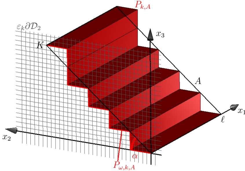
Figure 4.18: The face A and the polyhedral set P_{k,A}
