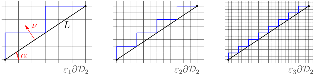
Figure 4.2: Approximation of a line segment along the scaled mesh \partial \mathcal{D}_2
