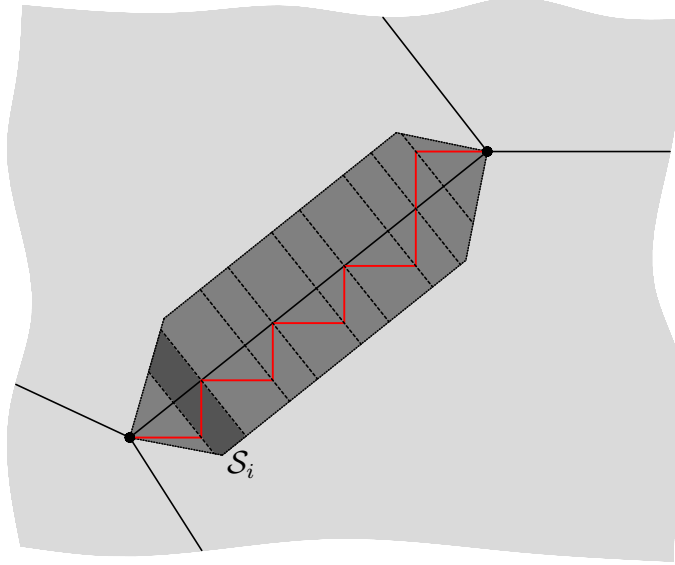
Figure 4.7: The subdomains \mathcal{S}_i of \mathcal{T}_{k,L}
