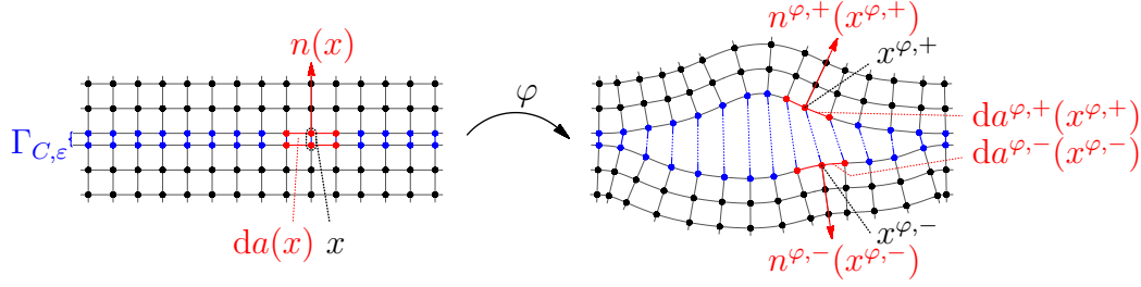
Figure 2.11: The backdriving force in the deformed configuration
