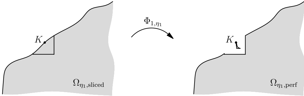
Figure 4.12: The sets \Omega_{\eta_1,\text{sliced}} and \Omega_{\eta_1,\text{perf}} around K \in \mathcal{K}_{\partial\Omega}(P_\psi)
