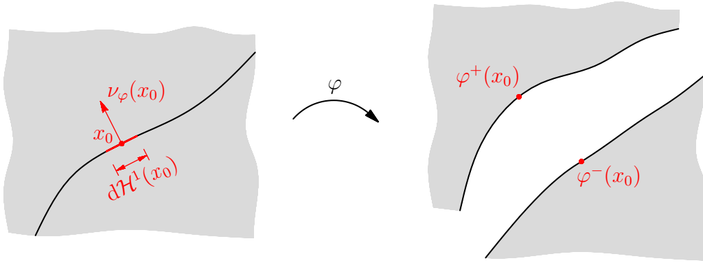
Figure 4.1: Geometry of the discontinuity set S_\varphi , locally around x_0
