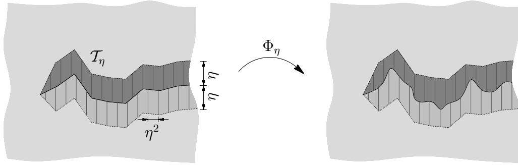
Figure 4.15: The pre-deformation \Phi_\eta|_{\mathcal{T}_\eta} : \mathcal{T}_\eta \rightarrow \mathcal{T}_\eta
