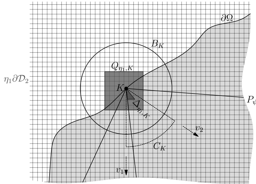
Figure 4.11: The geometrical situation of P_\psi in K \in \mathcal{K}_{\partial\Omega}(P_\psi)
