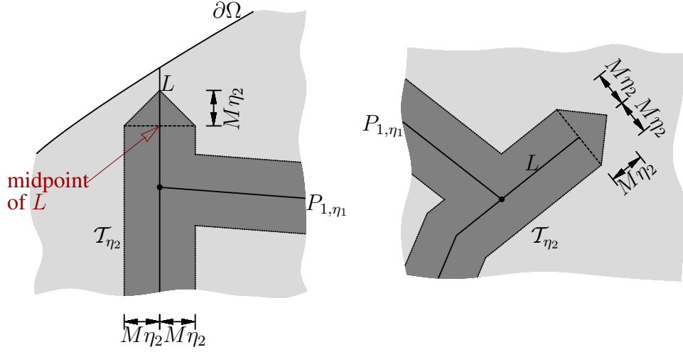
Figure 4.13: The tube \mathcal{T}_{\eta_2} and its construction over endpoints of P_{1,\eta_1} inside \Omega and near \partial\Omega
