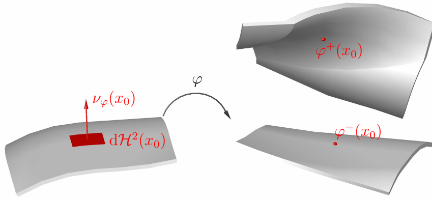
Figure 4.16: Geometry of the discontinuity set S_\varphi , locally around x_0
