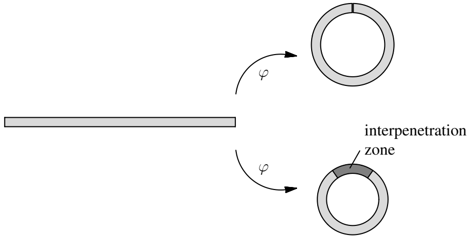
Figure 2.7: Deformation of a straight beam: contact and self-interpenetration
