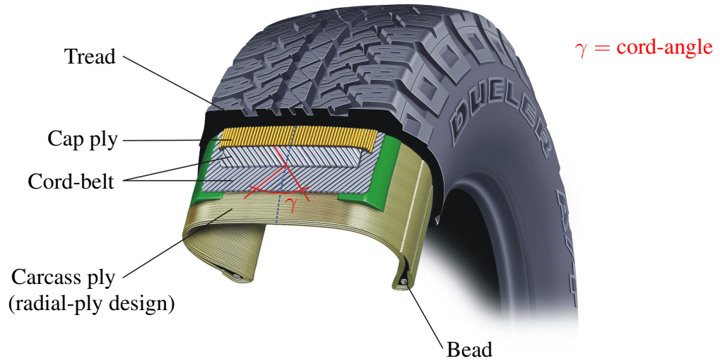
Figure 1.2: Structural elements of a pneumatic tire (courtesy of the Bridgestone Corporation)
